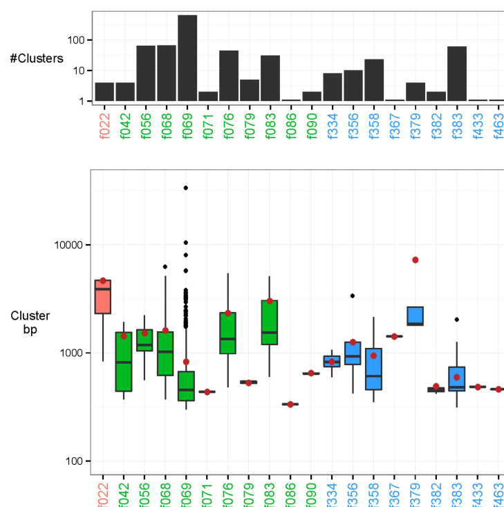
Figure 4. Unmappped clusters. The clusters are placed by their strongest associated feature. Feature types are marked in colour as follows: biological (red), methodological (green), and technical (blue). Top: Number of clusters associated to each feature on a log-10 scaled axis. There are 648 associated clusters of feature DNase/RNase: Promega DNase stop solution (f069), and 1 associated cluster to feature Polymerases: Phusion HF, NEB (f086). Bottom: Base-pair length (bp) of all cluster representatives (longest contig of each cluster) on a log-10 scaled axis. The N50 of all unmapped cluster representatives are marked by a brown dot. The longest cluster representative is 33.6 kb with N50 = 617 bp.
