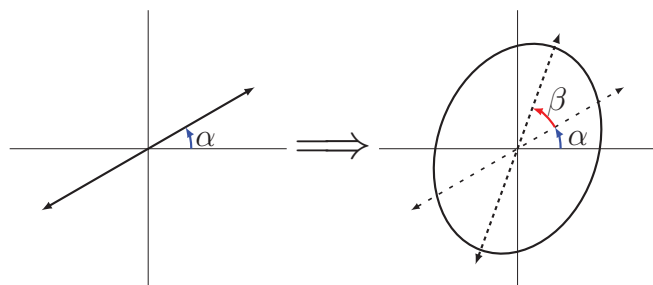
FIG. 1. Transformation of input linear polarization states (diagram on the left) to rotated elliptical output polarization states (diagram on the right). The angle of rotation \beta and the major to minor axis ratio (ellipticity) of the ellipse do not depend on the input angle \alpha .
