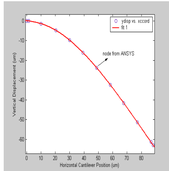
Figure 1 Smoothing spline fit of third position of cantilever deflection for sample 1.
