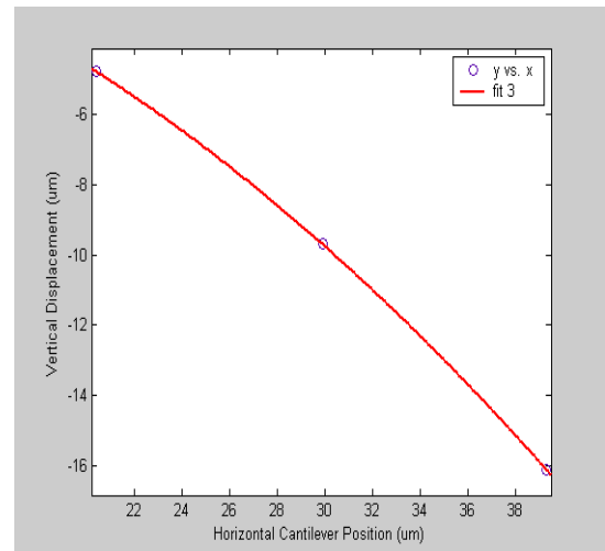
Figure 5. Quadratic fit for the second 3 data points for sample 1 at position 3
