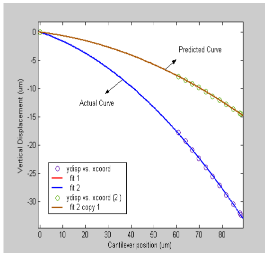
Figure 6. Actual Curve and Predicted Curve
