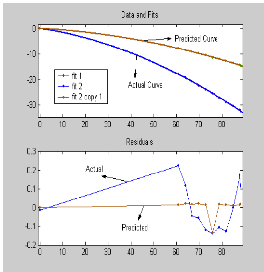
Figure 7. Data Fits and Residuals
