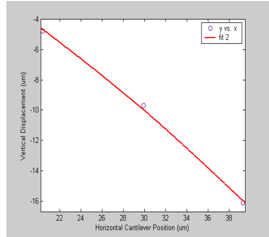
Figure 4. Spline fit for the second 3 data points for sample 1 at position 3
