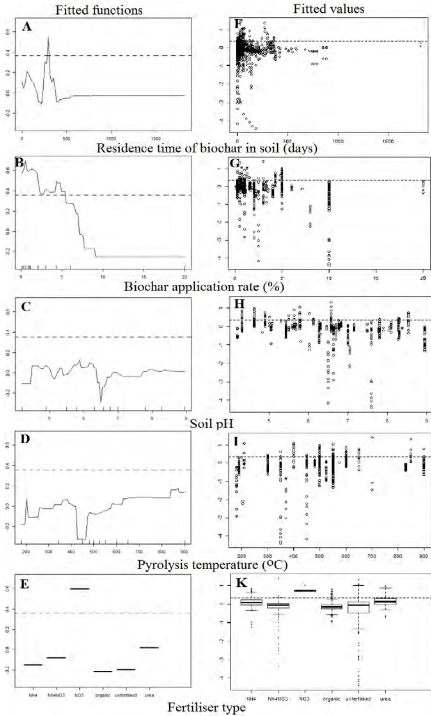
Figure S5: Partial dependence plots (A, B, C, D, E) and fitted values (F, G, H, I, K) showing the effects of biochar on soil \text{NO}_3^- -N. The fitted function shows the relationship between ES and an explanatory variable while all other explanatory variables are kept constant at their mean level.
