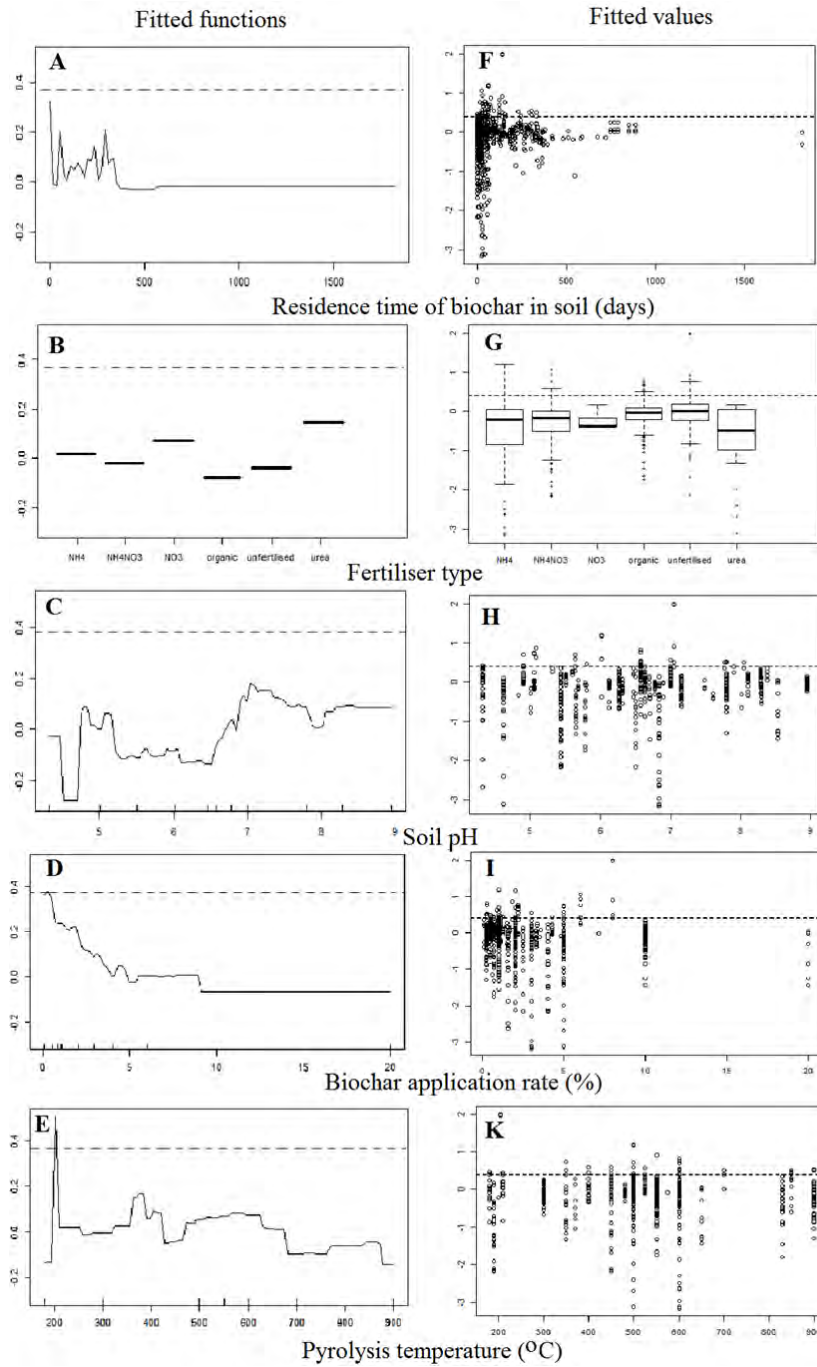
Figure S4: Partial dependence plots (A, B, C, D, E) and fitted values (F, G, H, I, K) showing the effects of biochar on soil \text{NH}_4^+\text{-N} . The fitted function shows the relationship between effect sizes and an explanatory variable while all other explanatory variables are kept constant at their mean level.
