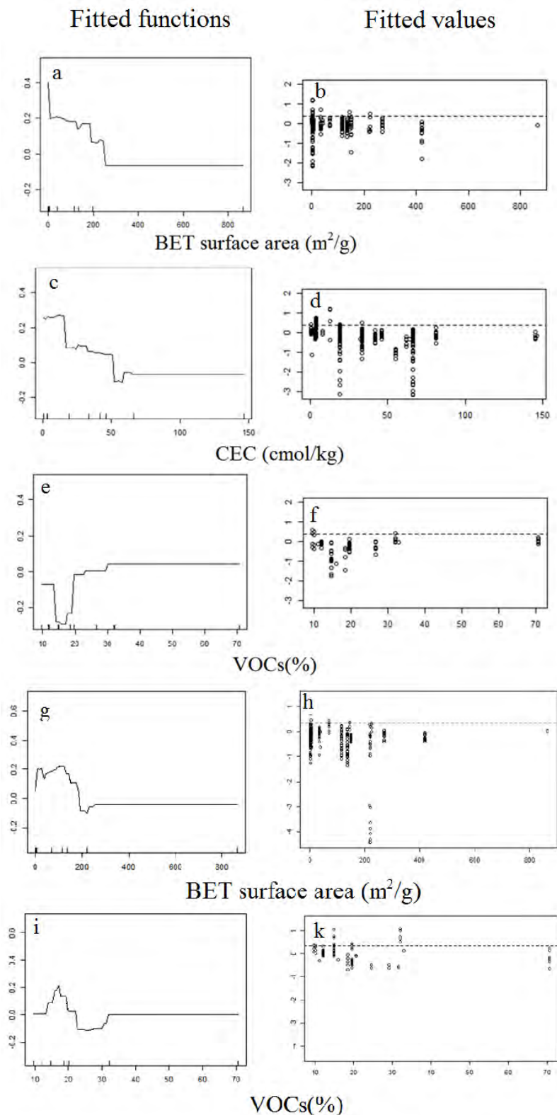
Figure 12: Partial dependence plots (a, c, e) and fitted values (b, d, f) showing the effects of biochar BET surface area, CEC, and VOCs on soil \text{NH}_4^+\text{-N} , and partial dependence plots (g, i) and fitted values (h, k) showing the effects of biochar BET surface area, and VOCs on soil \text{NO}_3^-\text{-N} . The fitted function shows the relationship between effect sizes and an explanatory variable while all other explanatory variables are kept constant at their mean level. The dashed lines showed no effect level.
