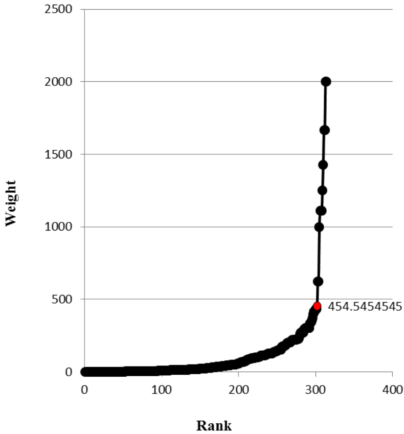
Figure S2: Weight-rank plot
