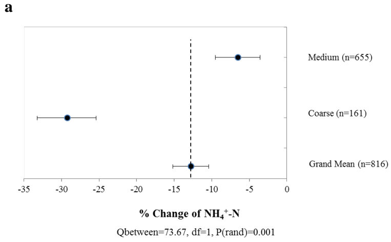
Figure 9: Influence of soil texture on \text{NH}_4^+ -N and \text{NO}_3^- -N availability in soil. Symbols represent mean effect sizes (percentage of change in \text{NH}_4^+ -N (a) and \text{NO}_3^- -N content (b)) with 95% confidence intervals. The numbers shown on the right correspond to observations in each class upon which the statistical analysis is based (n). The dotted line indicates the mean effect size for all soil texture types when biochar is co-applied to soil.
