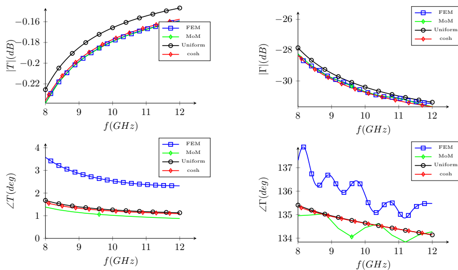
Figure 4. Magnitude and phase of the reflection \Gamma and transmission coefficient T from a strip with \sigma = 0.001 - j0.001 \text{ S m}^{-1} .
