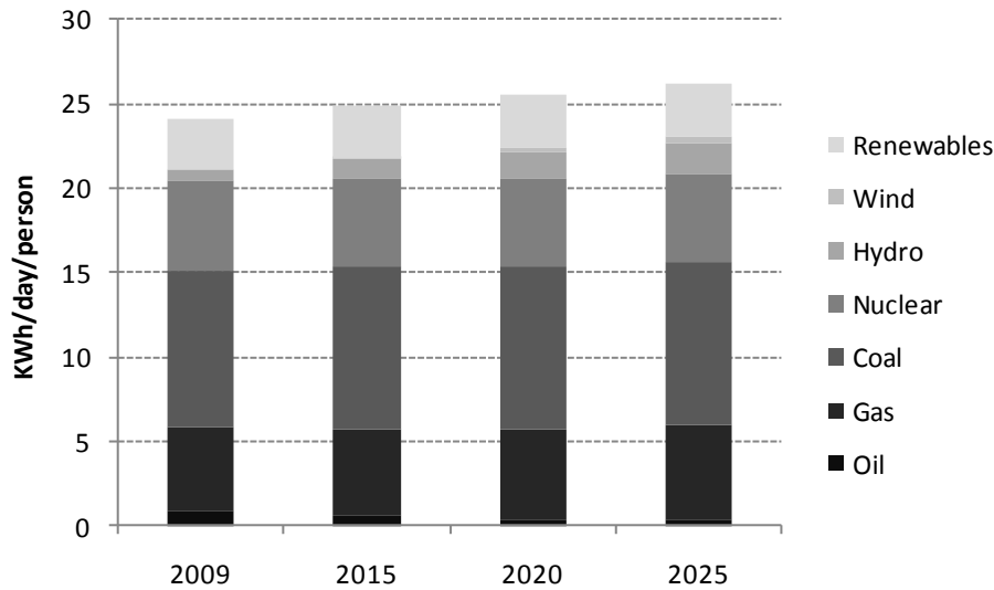
Figure 1: Forecast electricity consumption of developed countries 2009-2025 by generation type measured in power consumption per day per person. Assumes an energy intensity ceiling of -2% and efficiencies in gas, coal, oil and wind plants remain static.
