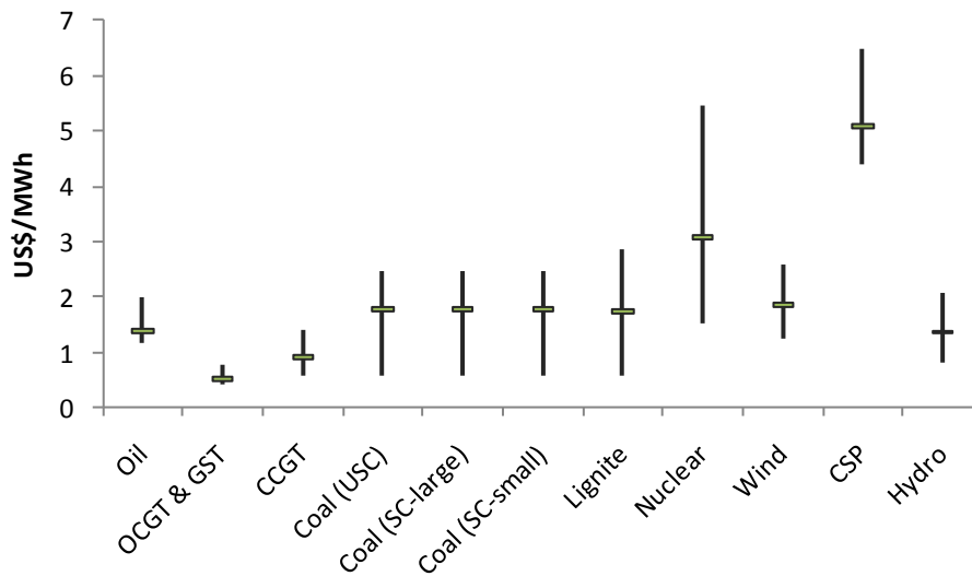
Figure 10: The high, low and average capital cost for different generation technologies in non-OECD countries 2010-2030 (US$/MWh). [OCGT – Open Cycle Gas Turbine, GST – Gas Steam Turbine CCGT – Combined Cycle Gas Turbine, USC – Ultra Super Critical, SC Super Critical, CSP – Concentrated Solar Power].
