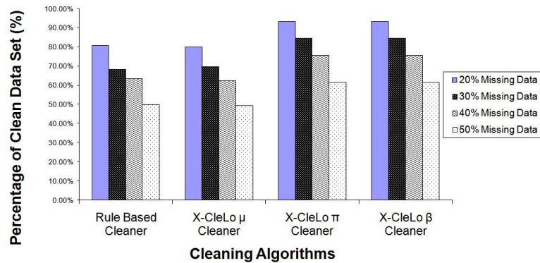
Fig. 6. The results of cleaning the Observation table with missing data present. Results are divided into the performance of the Rule Based and Clausal Defeasible Formulae ( \mu \pi and \beta ) when attempting to clean a database with 50%, 40%, 30% and 20% of the data missing.
