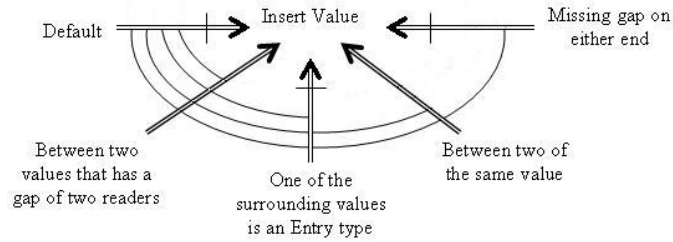
Fig. 4. The Logic Map created with the intent of detecting and inserting missing values.
