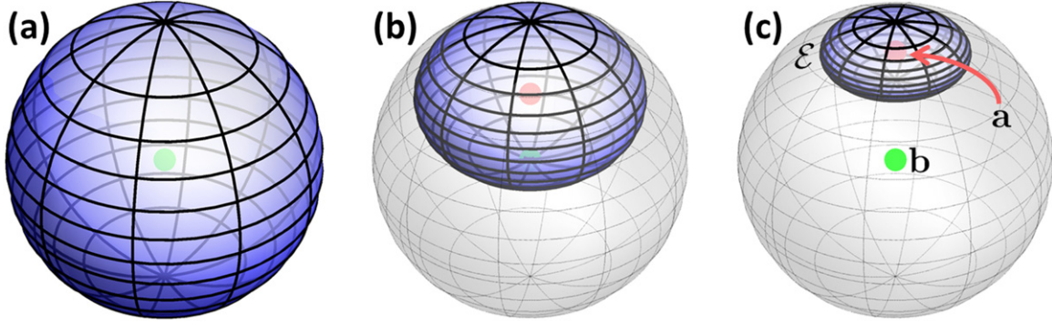
Figure 3. The geometric data for three maximal volume states \tilde{\rho}_c^{\max} with (a) c = 0 , (b) c = 0.5 and (c) c = 0.8 . Since these are canonical states we have \tilde{\mathbf{b}} = \mathbf{0} and \mathbf{c} = \mathbf{a} . Note that \mathcal{E} = \mathcal{E}_c^{\max} touches the North pole of the Bloch sphere for any c .
