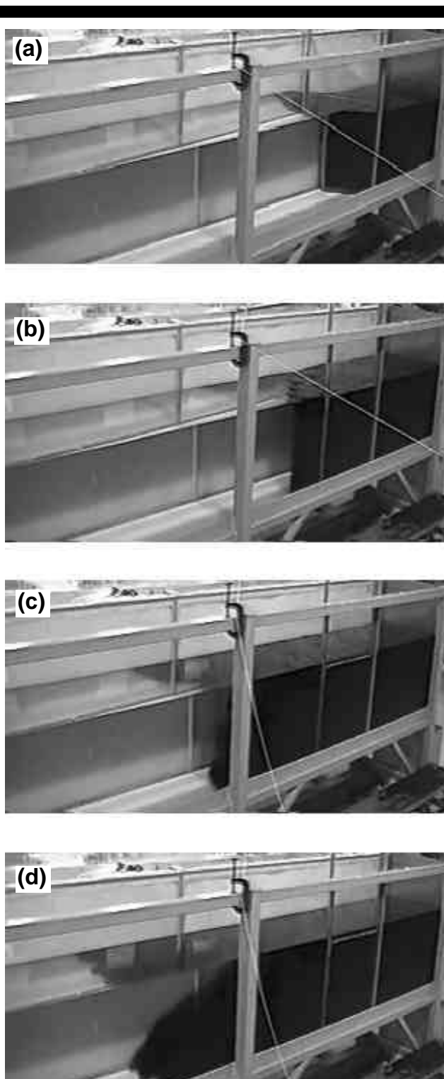
Figure 4. Spreading behaviour of a lock water into the tank for V = 0.24\text{ms}^{-1} and UT = 0.11\text{ms}^{-1} and H = 0.5\text{m} . The images were recorded at times corresponding to (a) 0.1 sec, (b) 3 sec (c) 6 sec and (d) 12 sec after the gate opening process commenced. NB. The spreading rate velocities are not presented in this paper.
