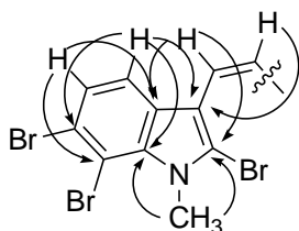
Figure 2 Key HMBC correlations for 1
