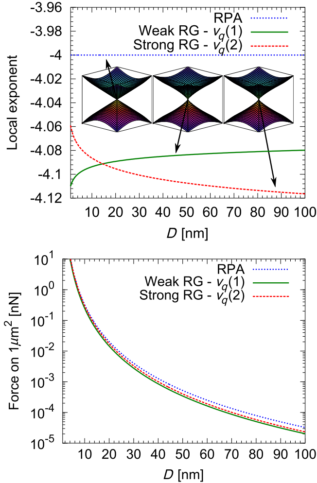
FIG. 3. Plot of the local exponent p(D) = (d \log |F| / d \log D) of the force (top, with band-structure inset) and the force F = (dE^{(2)}/dD) (bottom) using the RPA (dotted line), v_q^{(1)} [Eq. (4), solid line], and v_q^{(2)} [Eq. (5), with \beta = 2/\pi^2 , dashed line]. Here, we fix v = 10^5 m/s and \Lambda = 1/(1.42 \text{ \AA}) .
