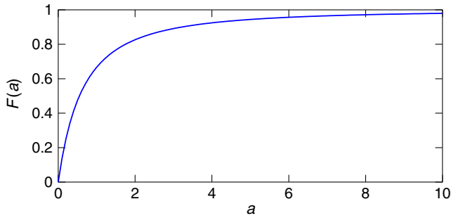
FIG. 1. Plot of the function F that controls, via Eq. (3), the value of the constant C_3 for the RPA van der Waals interaction between graphene sheets.
