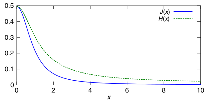
FIG. 2. Numerical fit [Eq. (12)] to the functions J(x) (solid line) and H(x) \equiv J(x)\sqrt{1+x^2} (dashed line) that control the magnitude of the self-energy and vertex corrections to the RPA beyond the simple renormalization of the velocity.
