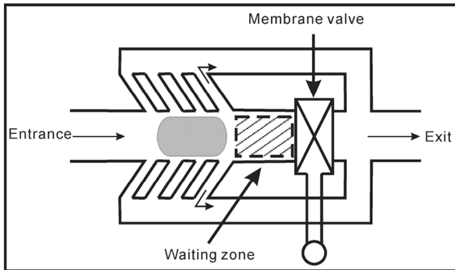
Fig. (14). Schematic illustration of pneumatically actuated droplet fusion device
