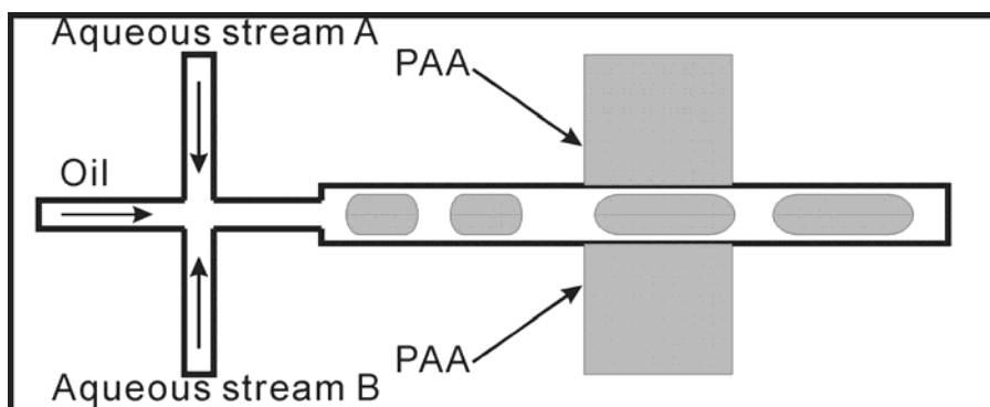
Fig. (6). Schematic illustration of surface-induced droplet fusion device
