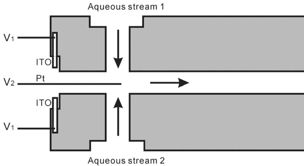
Fig. (10). Schematic illustration of microfluidic channel and electrode positions
