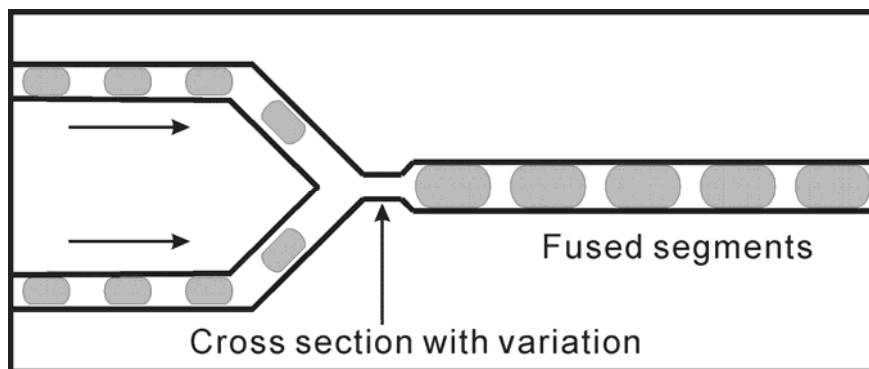
Fig. (2). Schematic illustration of fusion of droplets at a Y-junction
