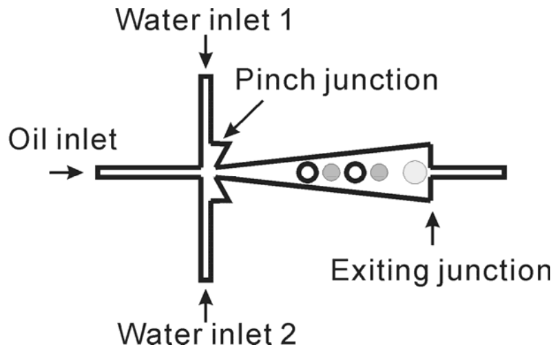
Fig. (4). Schematic illustration of the designed microchannel
