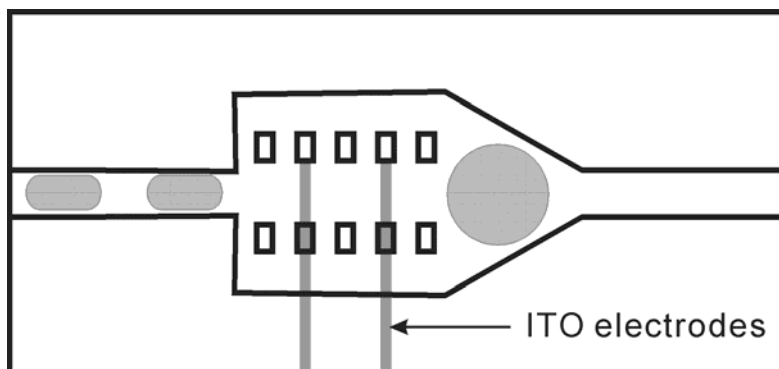
Fig. (8). Schematic illustration of the merging chamber with pillar arrays and embedded electrodes
