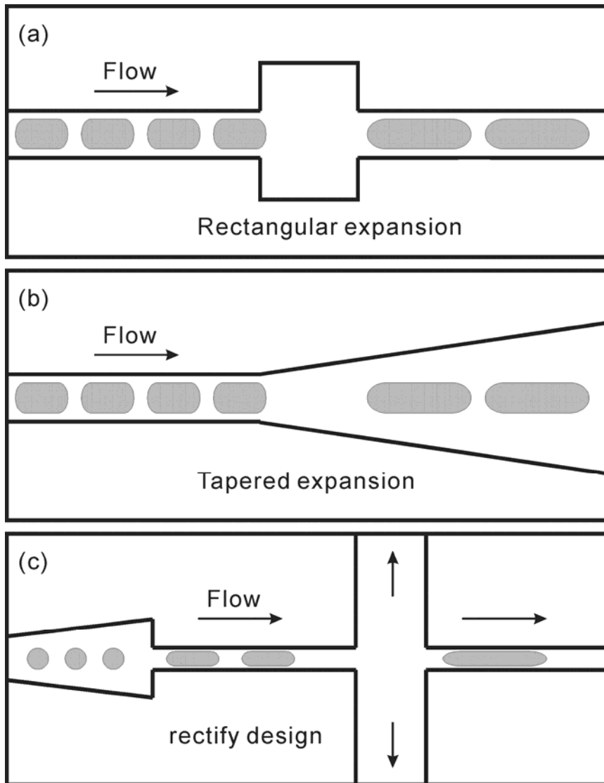
Fig. (3). Three different channel geometries. (a) Coalescence in channel with rectangular expansion, (b) Coalescence in channel with tapered expansion, (c) Coalescence in channel with rectification design
