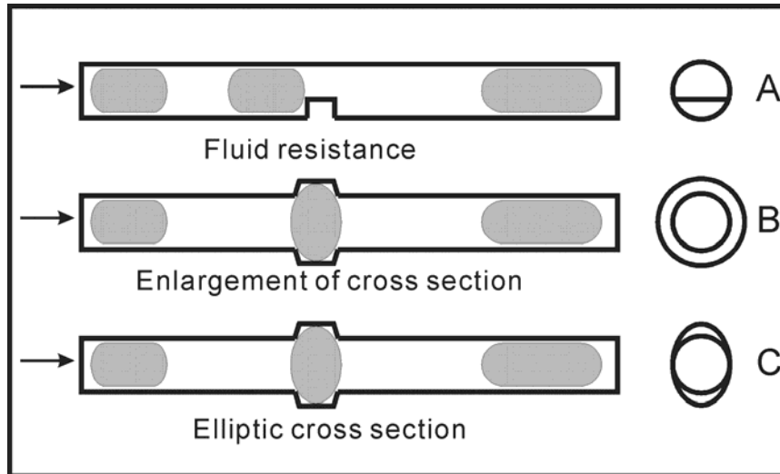
Fig. (1). Schematic illustration of fluid traps used in a microchannel. Cross sections are shown in the right: (A) wall step, (B) enlargement of cross section, (C) elliptic cross section
