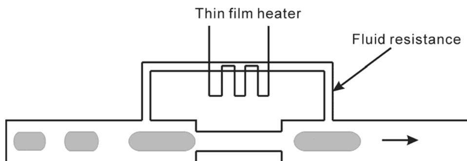
Fig. (11). Schematic illustration of thermally controlled droplet fusion microfluidic device
