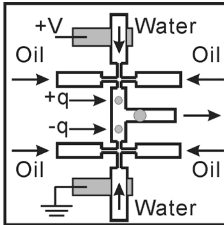
Fig. (7). Schematic illustration of electrocoalescence of droplets by applying an electric field through the aqueous stream
