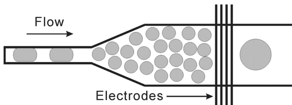
Fig. (9). Schematic illustration of the electrocoalescence behavior of a stream of water droplets under the effect of an applied electric field
