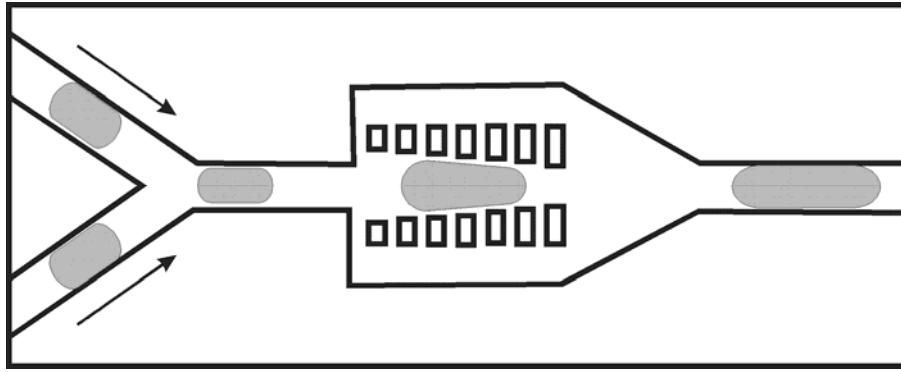
Fig. (5). Schematic illustration of pillar-induced droplet fusion device
