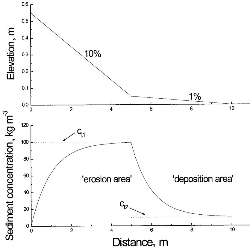
Fig. 1. Solutions to the unified erosion and deposition equations to show the downslope variation in sediment concentration as a result of a sudden decrease in slope steepness. See the text for parameter values used for this illustration.
