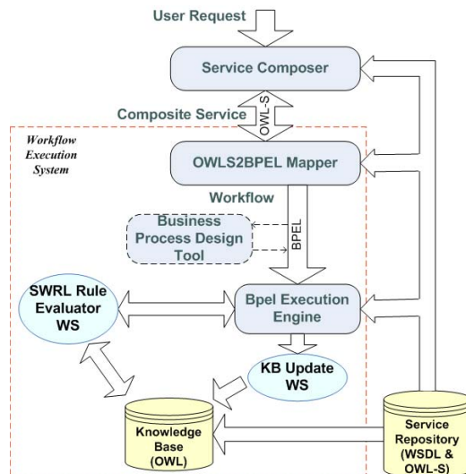
Figure 1. System Architecture
