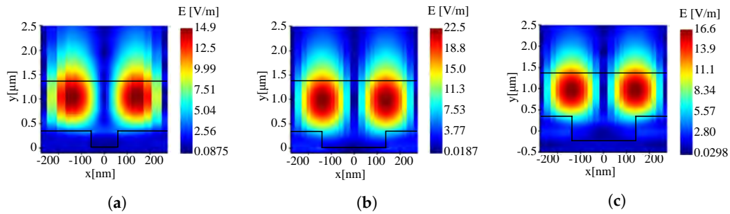
Figure 7. The electric field distributions for GMR gratings in EpoCore with different fill factors and grating heights: (a) FF=0.2 , d_{gr} = 350 nm, (b) FF=0.5 , d_{gr} = 350 nm and (c) FF=0.2 , d_{gr} = 600 nm.
