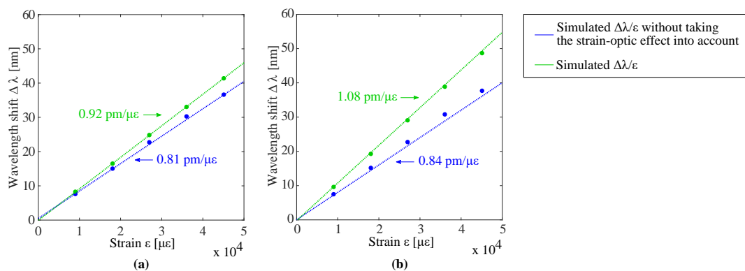
Figure 9. The simulated resonant wavelength shift \Delta \lambda as a function of the applied strain \epsilon for the GMR grating in (a) OrmoCore and (b) EpoCore. The used grating parameters are listed in Table 1.
