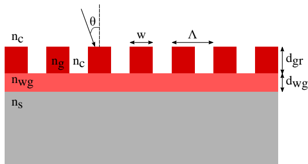
Figure 1. A schematic representation of a guided mode resonance (GMR) grating structure: A grating on top of a slab waveguide.
