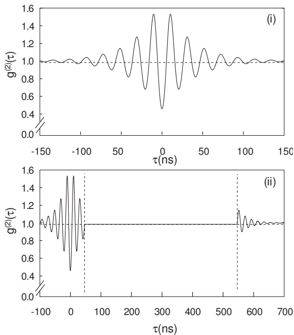
FIG. 4: (i) Time evolution of g^{(2)}(\tau) for (\Omega, g, \kappa, \gamma)/2\pi = (48.5, \sqrt{3}/8, 6.1, 4.9, 9.1) MHz. (ii) Time evolution of g^{(2)}(\tau) , for the same parameters as above, showing stabilization into a new steady state at time T_5 = 46.4 ns for a duration of 500 ns. The relative change in the driving strength \mathcal{E}'/\mathcal{E} = 0.9924
