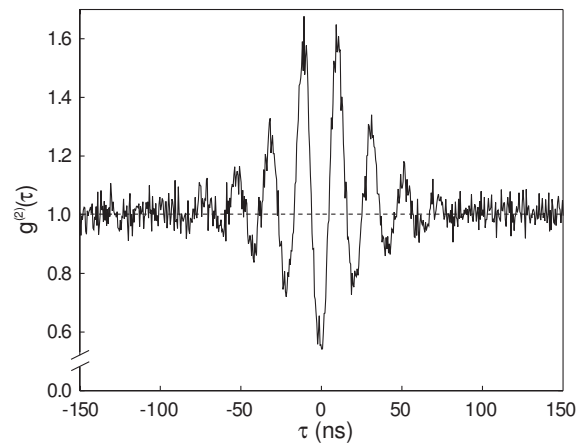
FIG. 8: Measured g^{(2)}(\tau) . \tau = 0 is defined by a photodetection in APD1. (\Omega, g, \kappa)/2\pi = (48.5, 6.1, 4.9) MHz. Data binned into 1.0 ns bins.
