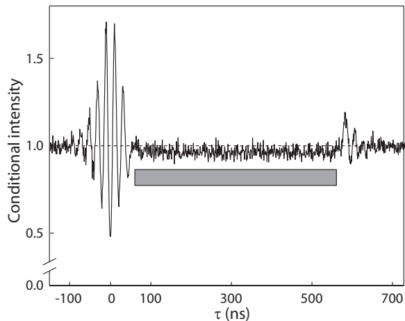
FIG. 9: Measured intensity correlation function. (\Omega, g, \kappa)/2\pi = (48.5, 6.1, 4.9) MHz. The grey box indicates the application time of the square feedback pulse, \Delta I = -2.7\% , \tau_{\text{fb}} = 45 ns, the intensity step was 500 ns long. Data binned into 1.0 ns bins.
