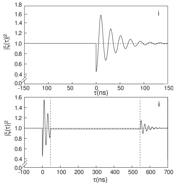
FIG. 1: (i) Time evolution of |\xi(\tau)|^2 for the semiclassical system when a forced jump is made at \tau = 0 for (\Omega, \kappa, \gamma)/(2\pi) = (48.5, 4.9, 9.1) MHz. (ii) Time evolution of |\xi(\tau)|^2 , for the same parameters as above, showing stabilization at time T_4 = 46.07 ns for a duration of 500 ns. The relative change in the driving strength is \mathcal{E}'/\mathcal{E} = 0.9922 .
