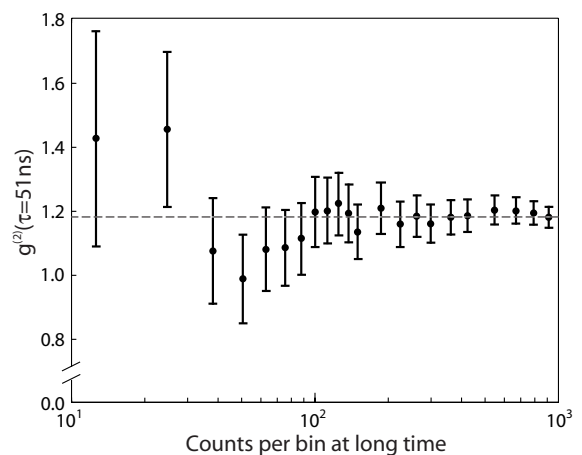
FIG. 12: Convergence of the \tau = 51 ns peak in Fig. 8 with increasing sample size. The value of g^{(2)}(\tau = 51 \text{ ns}) is plotted in a logarithmic scale against the average number of counts per bin at long time. Error bars are 1\sigma . The horizontal line passes through the final measured value of g^{(2)}(\tau = 51 \text{ ns}) .
