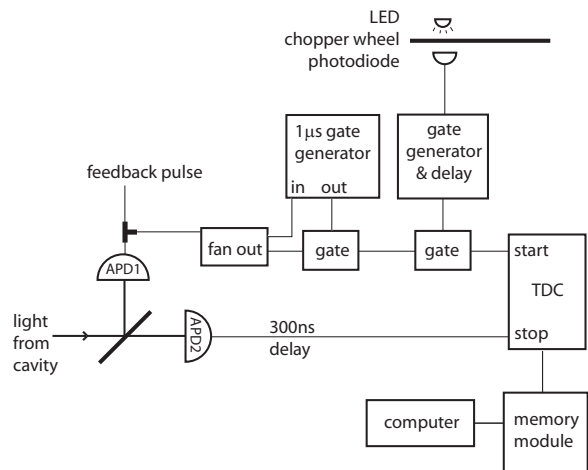
FIG. 7: Simplified diagram of correlation electronics. Electronic pulses produced by APD1 are split and used to initiate optical feedback and to start a TDC. The start pulses pass through two gates which ensures that the photon initiating an event did not originate from the cavity locking beam, and prevents the TDC from re-starting.
