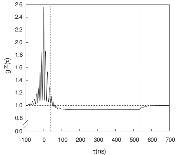
FIG. 3: g^{(2)}(\tau) for (\Omega, \kappa, \gamma, \Gamma)/(2\pi) = (48.5, 4.9, 6.0, 4.0) MHz, the same parameters as in Fig. 2.
