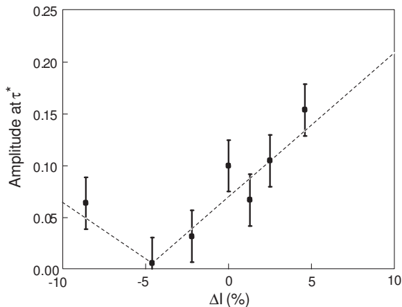
FIG. 13: Response of the system to feedback intensity steps of various sizes. \tau^* = 70 ns, (\Omega, g, \kappa)/2\pi = (37, 5.1, 3.7) . For this set, the optimal suppression occurs at \Delta I = -4.6\% . The dashed line is a theoretical prediction which includes the rise time of intensity step.
