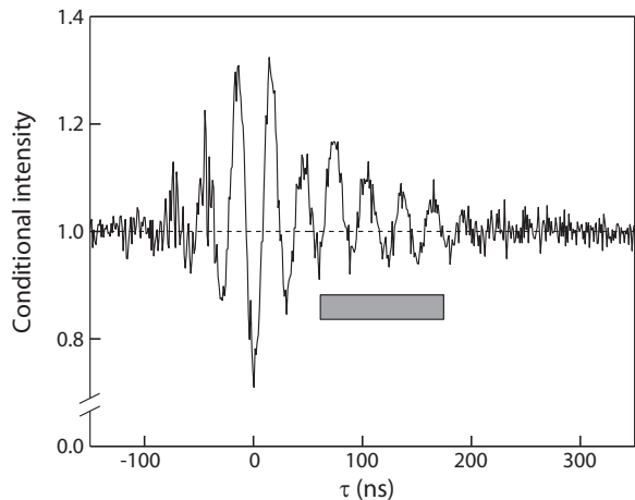
FIG. 10: Measured intensity correlation function. (\Omega, g, \kappa)/2\pi = (34, 5.1, 3.7) MHz. The grey box indicates the application time of the square feedback pulse, \Delta I = +3\% , \tau_{\text{fb}} = 56 ns, the intensity step was 120 ns long. The oscillation back to the steady state has been extended. Data binned into 1.0 ns bins.
