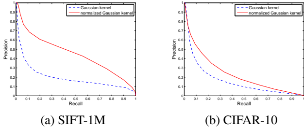
Figure 3. Precision-recall curves of k-NN search on SIFT-1M and CIFAR-10 when different distance metrics are compared.
