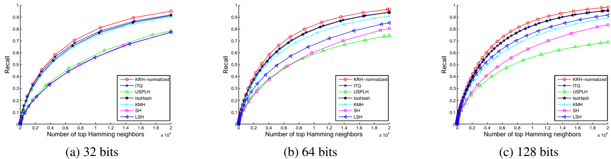
Figure 7. Recall curves of several unsupervised hashing methods on CIFAR-10.
