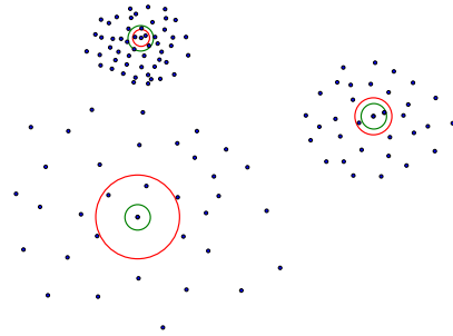
Figure 1. Illustration of the proposed normalized Gaussian kernel method (details are in Section 2). Red circle uses normalized Gaussian kernel on the retrieval radius, and green circle uses the Gaussian kernel. For a given threshold, the original Gaussian kernel gives the same retrieval radius. While using the normalized Gaussian kernel, the retrieval radius is adaptive to the surrounding distribution of the data points. This gives more consistent result for k -NN search.
