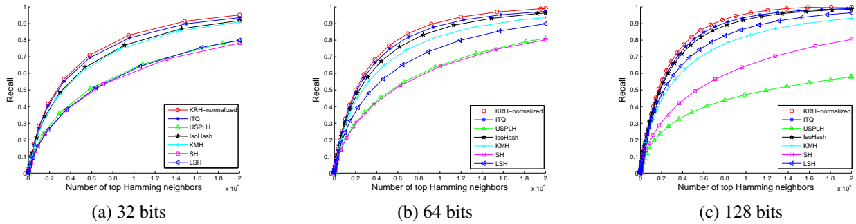
Figure 6. Recall curves of several unsupervised hashing methods on SIFT-1M.
