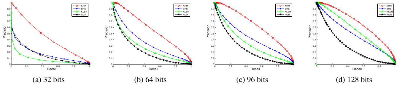
Figure 4. Precision-recall curves for kernel similarity preserving on SIFT-1M.
