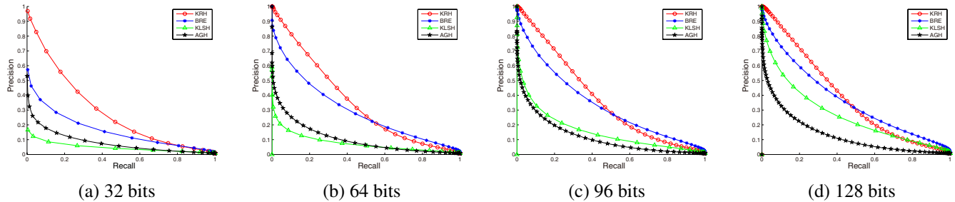
Figure 5. Precision-recall curves for kernel similarity preserving on CIFAR-10.
