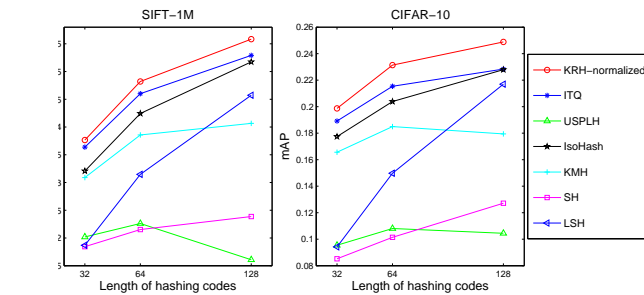
Figure 8. Mean averaged precision of several unsupervised hashing methods on SIFT-1M and CIFAR-10.
