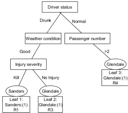
Figure 1. Tree for Accident address
