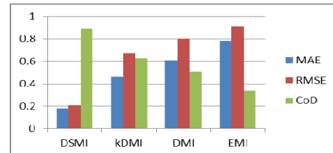
Figure 4. Categorical missing value imputation
