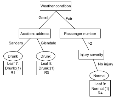
Figure 3. Tree for Driver status
