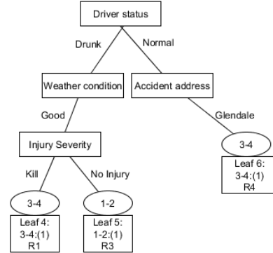
Figure 2. Tree for Passenger number
