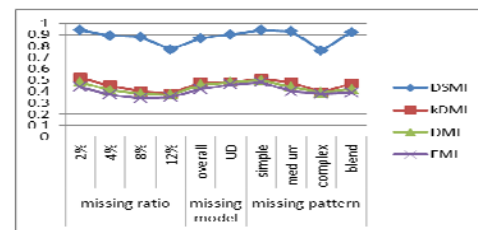
Figure 5. Average performance based on coefficient of determination (CoD)
