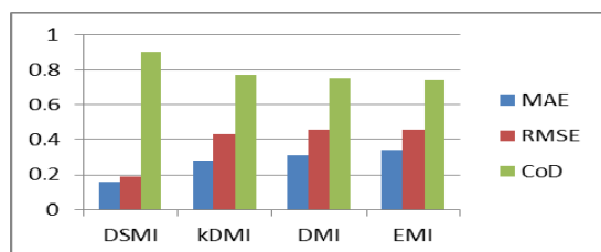
Figure 6. Numerical missing value imputation
