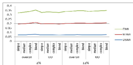
Figure 7. Average performance based on RMSE
