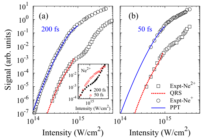
FIG. 3. Double- and single-ionization yields for Ne exposed to linearly polarized laser pulses at 800 nm with pulse durations of (a) 200 fs and (b) 50 fs. The experimental data shown in panels (a) and (b) are taken from Larochelle et al. [41] and Bhardwaj et al. [16], respectively. The simulated results from the QRS model for double ionization and the PPT model for single ionization are normalized for good visual agreement with experiment. The calculations include the integration over the focal volume of the laser. The inset shows the measured knee structure in the double-ionization yield for 200 and 50 fs pulses, respectively.
