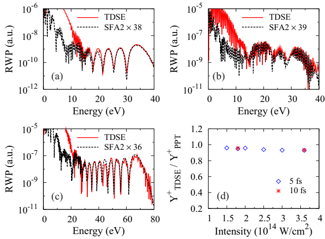
FIG. 4. Comparison of the returning electron wave packets from TDSE and SFA2 for Ne in a linearly polarized 800-nm laser field with parameters of (a) 5 fs and 1.8 \times 10^{14} W/cm 2 , (b) 10 fs and 1.8 \times 10^{14} W/cm 2 , and (c) 5 fs and 3.6 \times 10^{14} W/cm 2 . Panel (d) shows the ratio of the single-ionization yield from TDSE ( Y_{\text{TDSE}}^+ ) over the single-ionization yield of PPT ( Y_{\text{PPT}}^+ ) for Ne in a linearly polarized 800-nm laser field as a function of intensity for pulse durations of 5 and 10 fs, respectively. In panels (a)–(c), the returning electron wave packets of SFA2 are renormalized according to the corresponding TDSE results.
