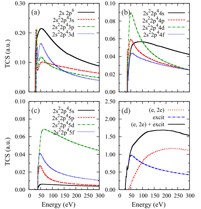
FIG. 1. Total cross sections for electron-impact ionization and excitation of \text{Ne}^+ from the ground state. Excitation of the configurations (a) 2s2p^6 , 2s^22p^43s , 2s^22p^43p , and 2s^22p^43d ; (b) 2s^22p^44s , 2s^22p^44p , 2s^22p^44d , and 2s^22p^44f ; (c) 2s^22p^45s , 2s^22p^45p , 2s^22p^45d , and 2s^22p^45f . Panel (d) shows the summed total cross sections for ionization and excitation of all configurations in panels (a)–(c).
