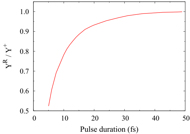
FIG. 6. Pulse-duration dependence of the ratio between the total yield of returning electrons Y^R and the total yield of single ionization Y^+ for Ne in an 800-nm pulse at a peak intensity of 6.0 \times 10^{14} \text{ W/cm}^2 . The ratio Y^R/Y^+ is normalized to unity at 50 fs. See text for details.
