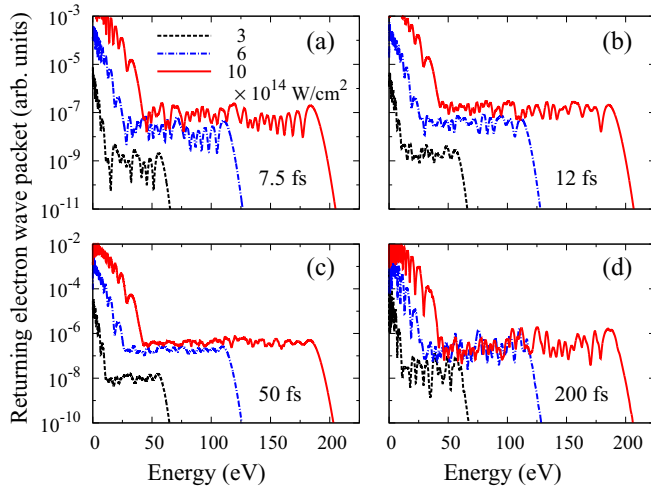
FIG. 2. Returning electron wave packets W_R(E_r) for Ne in linearly polarized 800-nm laser fields with pulse durations of (a) 7.5 fs, (b) 12 fs, (c) 50 fs, and (d) 200 fs at single peak intensities of 3, 6, and 10 \times 10^{14} W/cm 2 , respectively. The sharp rapid oscillations in the returning electron wave packets were smoothed out to improve the visibility.
