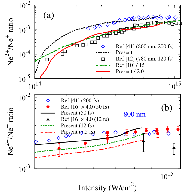
FIG. 5. Ratio between double and single ionization as a function of intensity for Ne exposed to linearly polarized laser pulses with (a) pulse duration of 200 fs at a wavelength of 800 nm and pulse duration of 120 fs at a wavelength of 780 nm, and (b) pulse durations of 7.5, 12, 50, and 200 fs at a wavelength of 800 nm. In panel (a), the present simulations are compared with the experimental data of Larochelle et al. [41] and Sheehy et al. [12], as well as with the S -matrix calculations of Becker and Faisal [10]. In panel (b), the present results are compared with the experimental data of Bhardwaj et al. [16]. See text for details.
