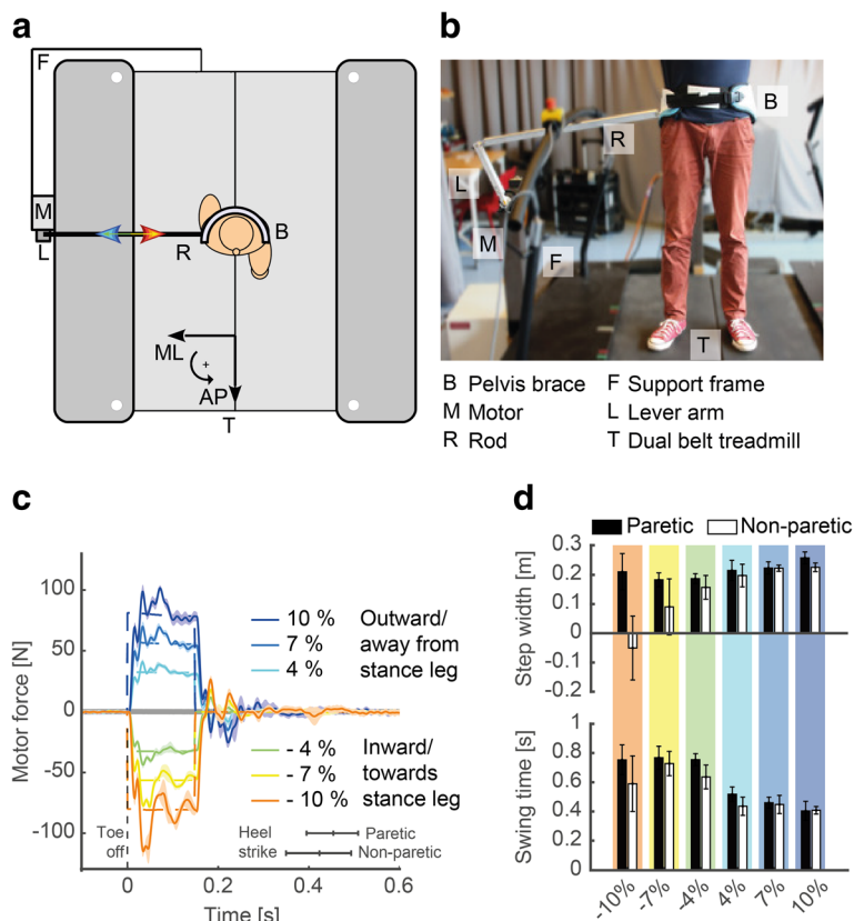
Fig. 2 To systematically assess how patients maintain their balance when being perturbed during walking, the University of Twente has developed a pelvic perturbation device ( a and b ) [38]. This device consists of an admittance-controlled motor (Moog, Nieuw Venne, the Netherlands) connected via a lever arm and a rod to a pelvic brace worn by the subject. The device allows providing perturbations in different directions, with different magnitudes and different durations at precisely timed instances of the gait cycle while walking on a treadmill ( c , mediolateral perturbations timed at toe off with magnitudes expressed as % of body weight). In collaboration with Roessingh Research & Development, the device was used to assess the foot placement strategies of ambulatory stroke survivors when being perturbed away or towards the stance leg at the start of swing of the paretic or non-paretic legs. Responses of the step directly following the perturbation in a single stroke survivor are indicated in ( d ). Whereas the stroke survivor made a cross step, as evidenced by the negative step width, with his non-paretic leg when being forcefully perturbed towards the paretic leg, he did not make a cross step with his paretic leg. When being perturbed away from the stance leg, both the paretic and non-paretic side only slightly adjusted the step width but the foot was placed faster on the ground, as evidenced by the decreased swing time, to counteract the perturbation
