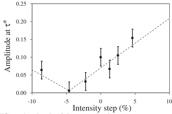
FIG. 4. Amplitude of the normalized intensity response at time \tau^* (first oscillation extreme of g^{(2)}(\tau) after the application of the feedback pulse) as a function of the size of the feedback step. The dashed line is a theoretical prediction.
