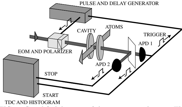
FIG. 2. Simplified diagram of the experimental setup. The output of the cavity QED system passes through a beam splitter (entrance of an intensity correlator) such that the detection of a photon at the “start” avalanche photodiode (APD) also triggers a change in the driving intensity through a pulse that drives an electro-optical modulator EOM in front of a polarizer. A histogram of the delays between the “start” and “stop” gives the conditional evolution of the intensity
