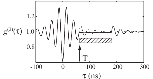
FIG. 1. Conditional evolution of cavity QED system with (continuous line) and without (dashed line) feedback. The shaded rectangle region corresponds to an instantaneous step down of 0.2 % of the driving intensity applied at time T .
