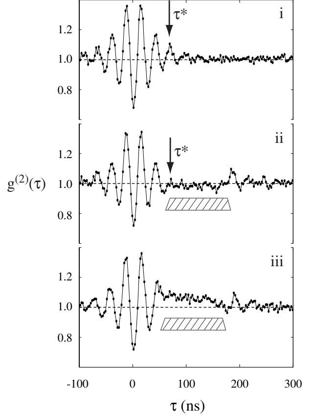
FIG. 3. Measured intensity correlation function with the feedback step applied during the shaded region: i) no feedback ( g\sqrt{N}/2\pi = 37 MHz), ii) suppression with a step down change of 2.6 % ( g\sqrt{N}/2\pi = 37 MHz) iii) suppression with a step up change of 3.9% ( g\sqrt{N}/2\pi = 31 MHz). The oscillation of the system continues with the same phase and amplitude once the step is off. Note that the time T for the beginning of the feedback in ii and iii is different as indicated by the position of the shaded region. The data has been binned in 2.5 ns points joined with a line.
