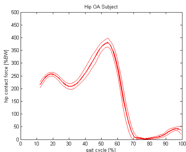
Figure 3: Right hip Joint Contact Force for the hip OA subject during walking. The thick red line is the average from the 10 walking trials while the thin red line represents 1 standard deviation. Peak HCF occurs at around 55% of the gait cycle.
