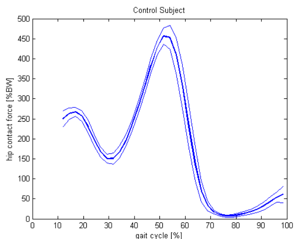
Figure 2: Right hip joint contact force for the control subject during walking. The thick blue line is the average from the 10 walking trials while the thin blue line represents 1 standard deviation. Peak HCF occurs at around 55% of the gait cycle.
