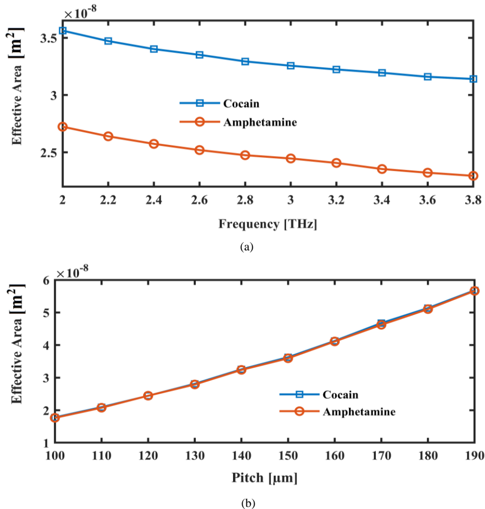
Figure 9. Demonstrates the correlation between the effective area ( A_{eff} ) of the chosen monitoring material and (a) the frequency indication at a specific pitch of 120 \mu\text{m} , and (b) the pitch variation with a constant frequency of 3 THz
