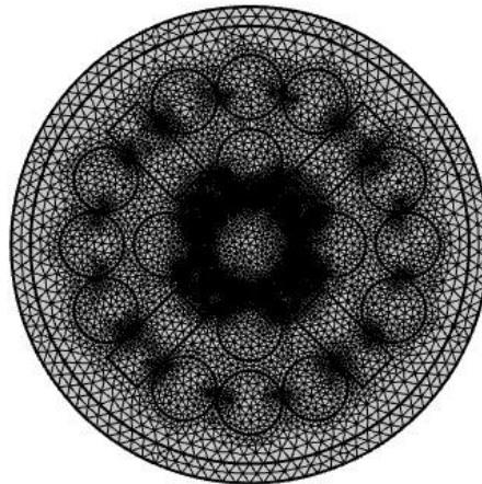
Figure 1. Recommended PCF mesh presentation
