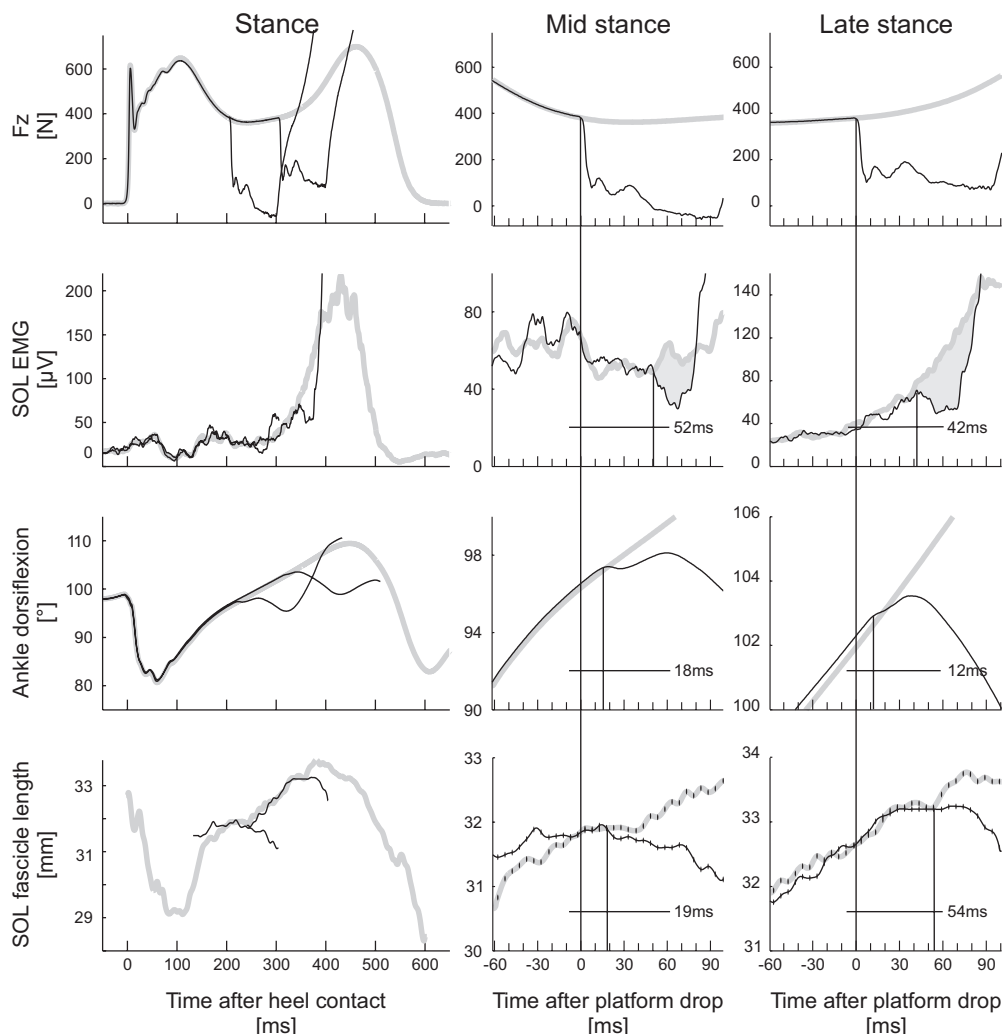
FIG. 3. Ensemble-averaged ( n > 30 ) vertical ground reaction force (Fz), soleus activity (SOL EMG, low-pass 40 Hz), ankle excursion, and soleus muscle fascicle length ( n = 3 ) for a representative subject shown for the stance phase (left column) and for a window ( -60 to 100 ms) surrounding the mid- and late-stance perturbations (middle and right columns, respectively). The vertical lines indicate the first major deflection from the ensemble average of the control steps for vertical ground reaction force (GRF), soleus EMG, ankle movement, and fascicle length (visual inspection). The latency from the drop of the platform to the onset of the unload response (gray area), ankle movement, and fascicle shortening are indicated to the right.
