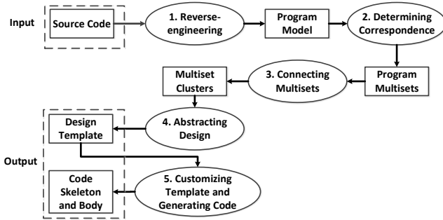
Fig. 2. Approach Overview
