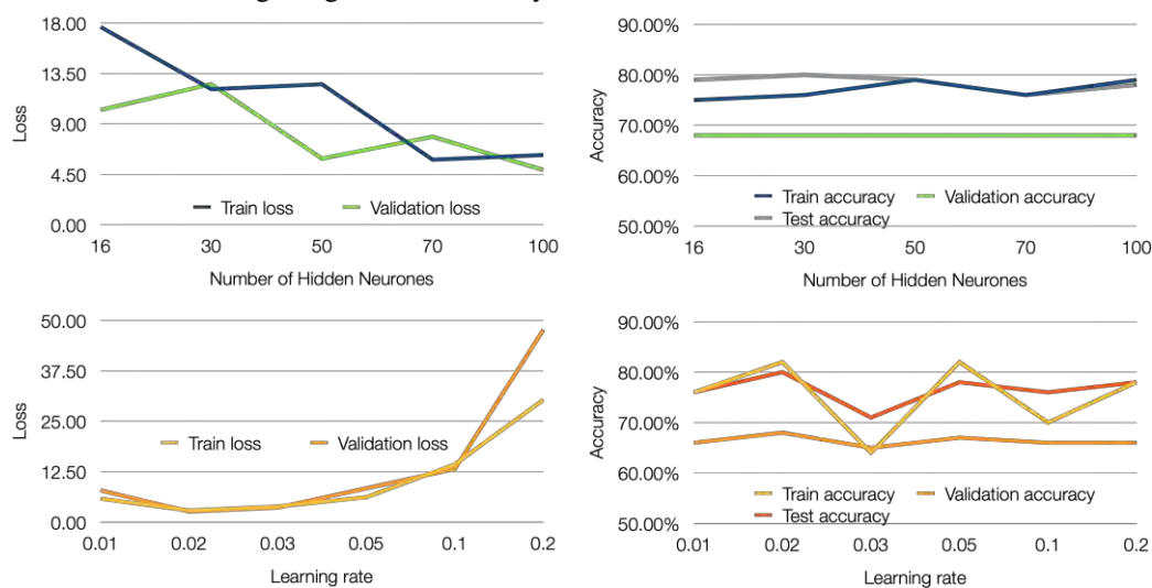
Figure 7: GCN Tuning
