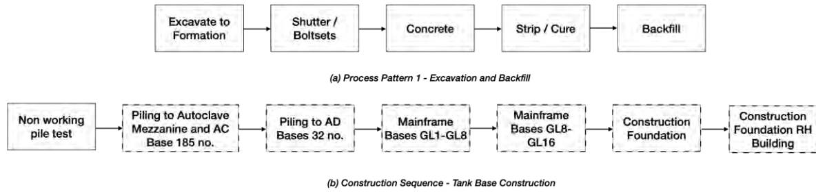
Figure 8: Method patterns – Results
