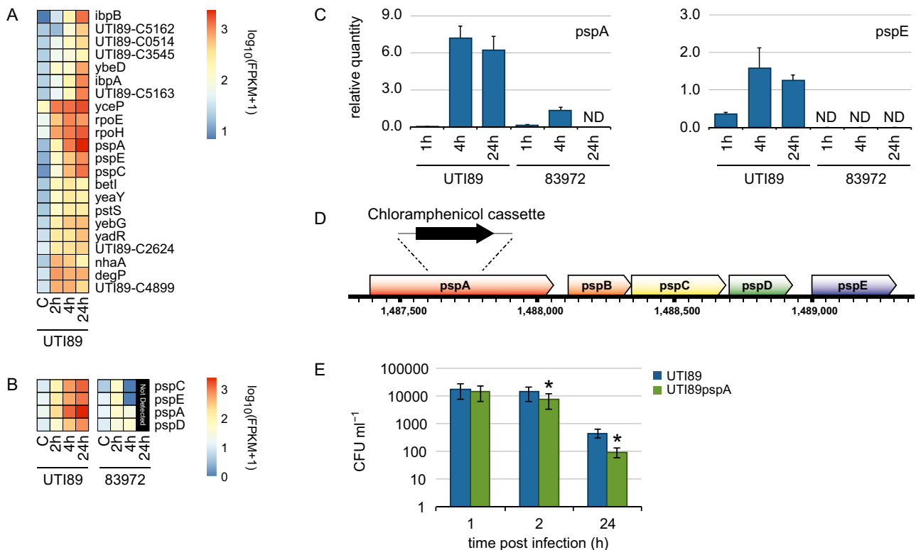
Fig. 6. UPEC genes associated with intramacrophage survival.
