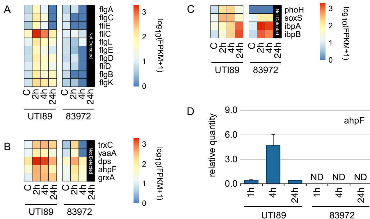
Fig. 5. Regulation of UPEC flagella, OxyR regulon and hydrogen peroxide-induced genes in the intramacrophage environment. A–C. Heat maps summarizing the RNA-Seq-derived expression profiles of flagellar genes (A), OxyR regulon genes (B) and hydrogen peroxide-induced genes (C). All values are log-transformed FPKM counts. D. Bar plot showing the relative mRNA levels of ahpF , as determined by RT-qPCR. qPCR data represent mean relative expression \pm range ( n = 2 ) of two biological replicates; ND, not detected.
