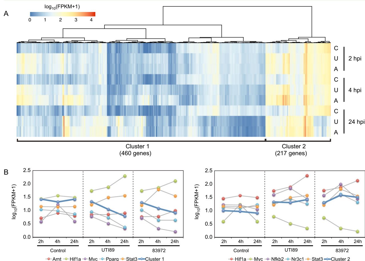
Fig. 3. Transcription factors associated with DE BMM genes.
