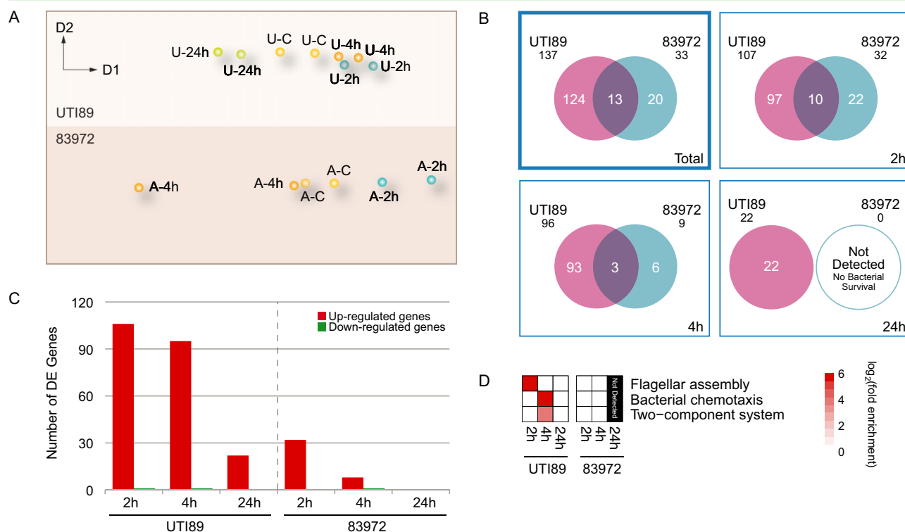
Fig. 4. UPEC transcriptome analysis.
