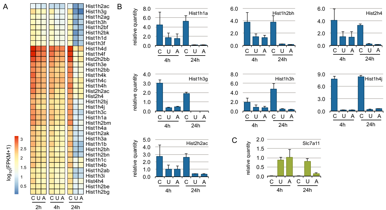
Fig. 2. Gene regulation in BMM.
