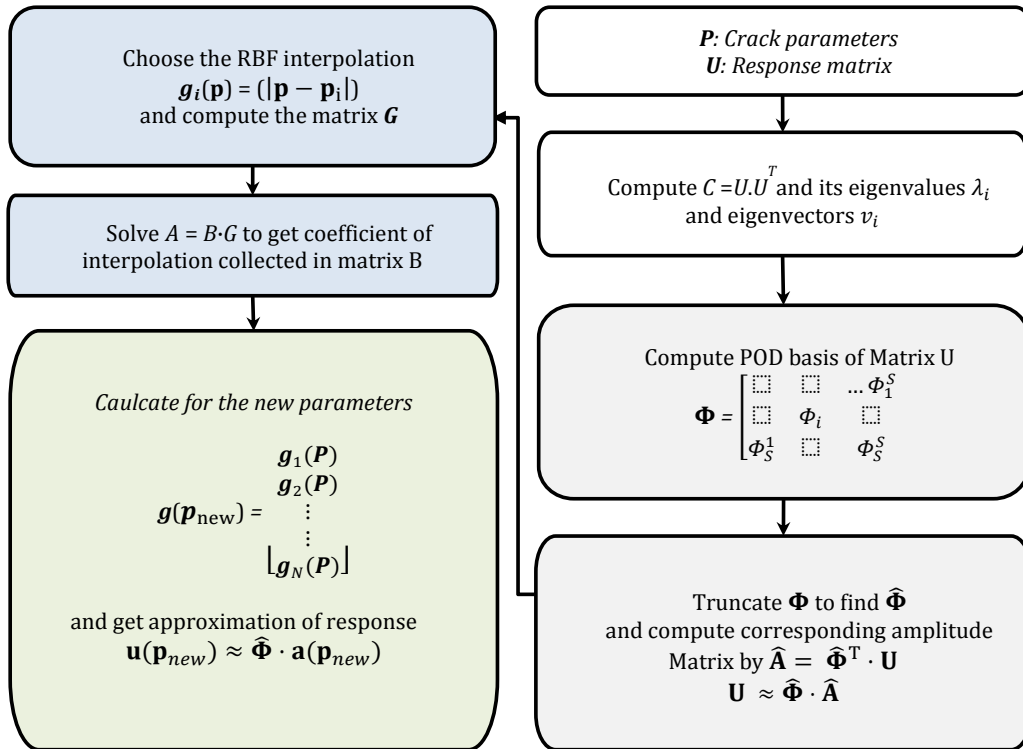
Figure 5. POD-RBF methodology
