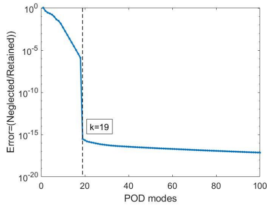
Figure 14. The truncation point on the dynamic model
