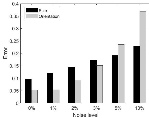
Figure 10. Effect of noise level on the average prediction error for all cracks
