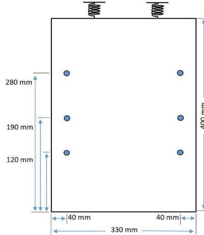
Figure 12. Plate dimensions and accelerometer positions
