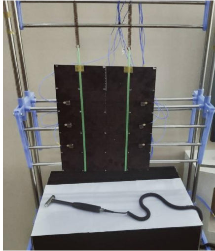
Figure 13. Experimental setup.
