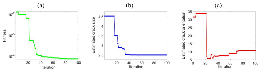
Figure 9. C2 Crack identification
