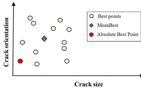
Figure 1. Illustration of the MeanBest point.
