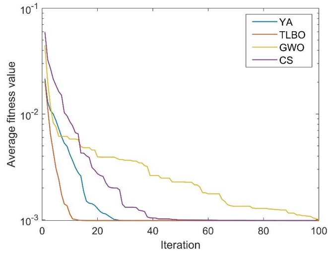
Figure 17. Average fitness convergence by YA, TLBO, GWO, and CS algorithms in C14
