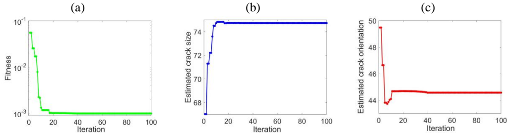
Figure 16. C14 crack parameter identification versus iterations
