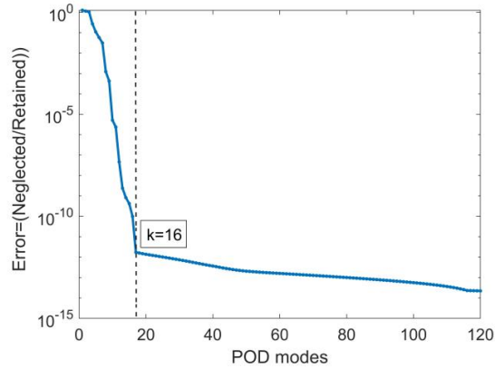
Figure 7. The truncation point on the Elastostatic model
