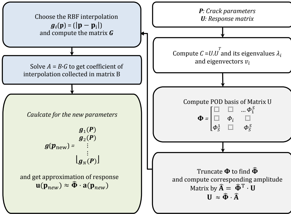
Figure 5. POD-RBF methodology
