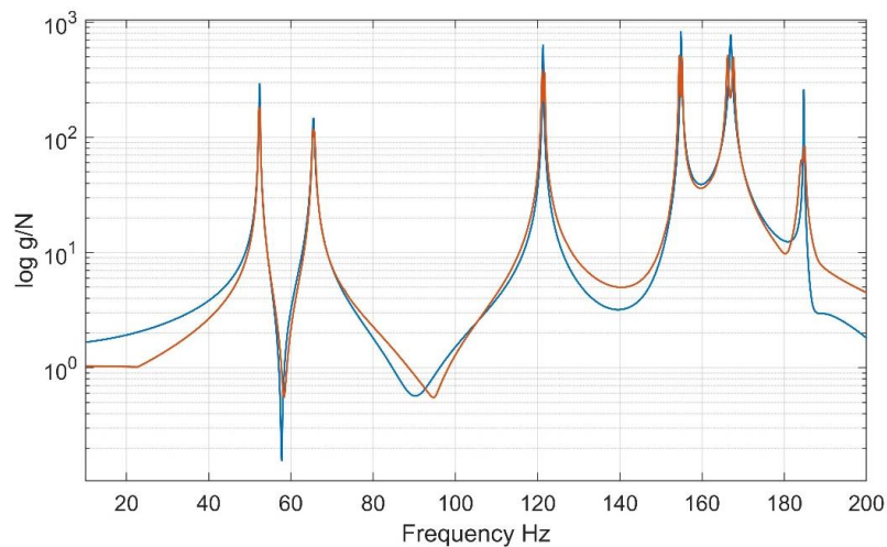
Figure 15. Experimental FRF from 25 mm crack at 45^\circ vs. predicted using POD-RBF
