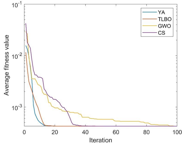
Figure 11. Average fitness convergence by YA, TLBO, GWO, and CS algorithms in C8
