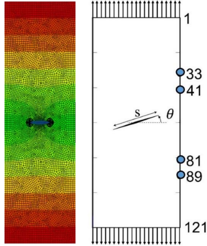
Figure 6. Cracked specimen
