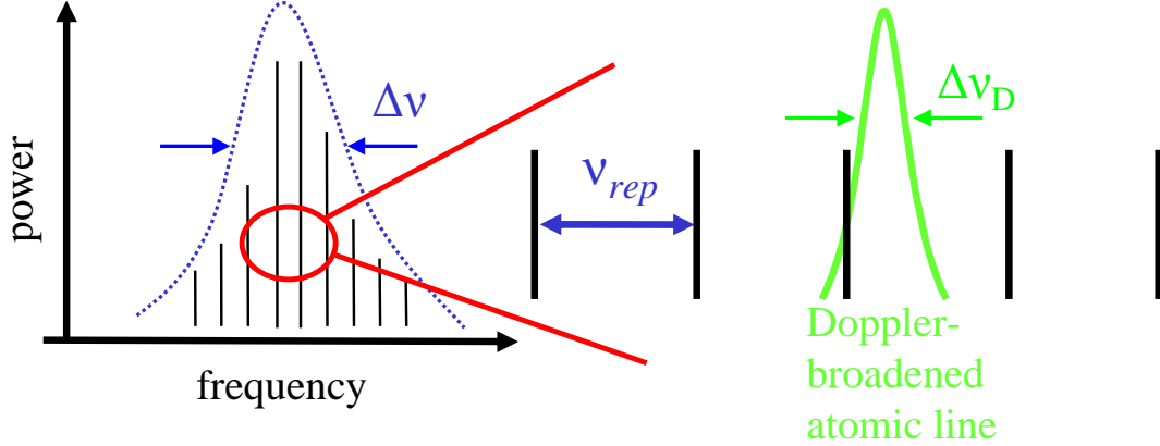
FIG. 1: Velocity-selective scattering with a high-repetition-rate pulse train. Left: Optical spectrum generated by a mode-locked pulse train, consisting of equally spaced sharp lines (black) with a spectral envelope of bandwidth \Delta\nu (blue). Right: Velocity selective scattering occurs when one laser line is nearly resonant with a Doppler-broadened atomic transition of width \Delta\nu_D . For repetition rate \nu_{\text{rep}} \ll \Delta\nu_D , all other laser lines induce negligible scattering.
