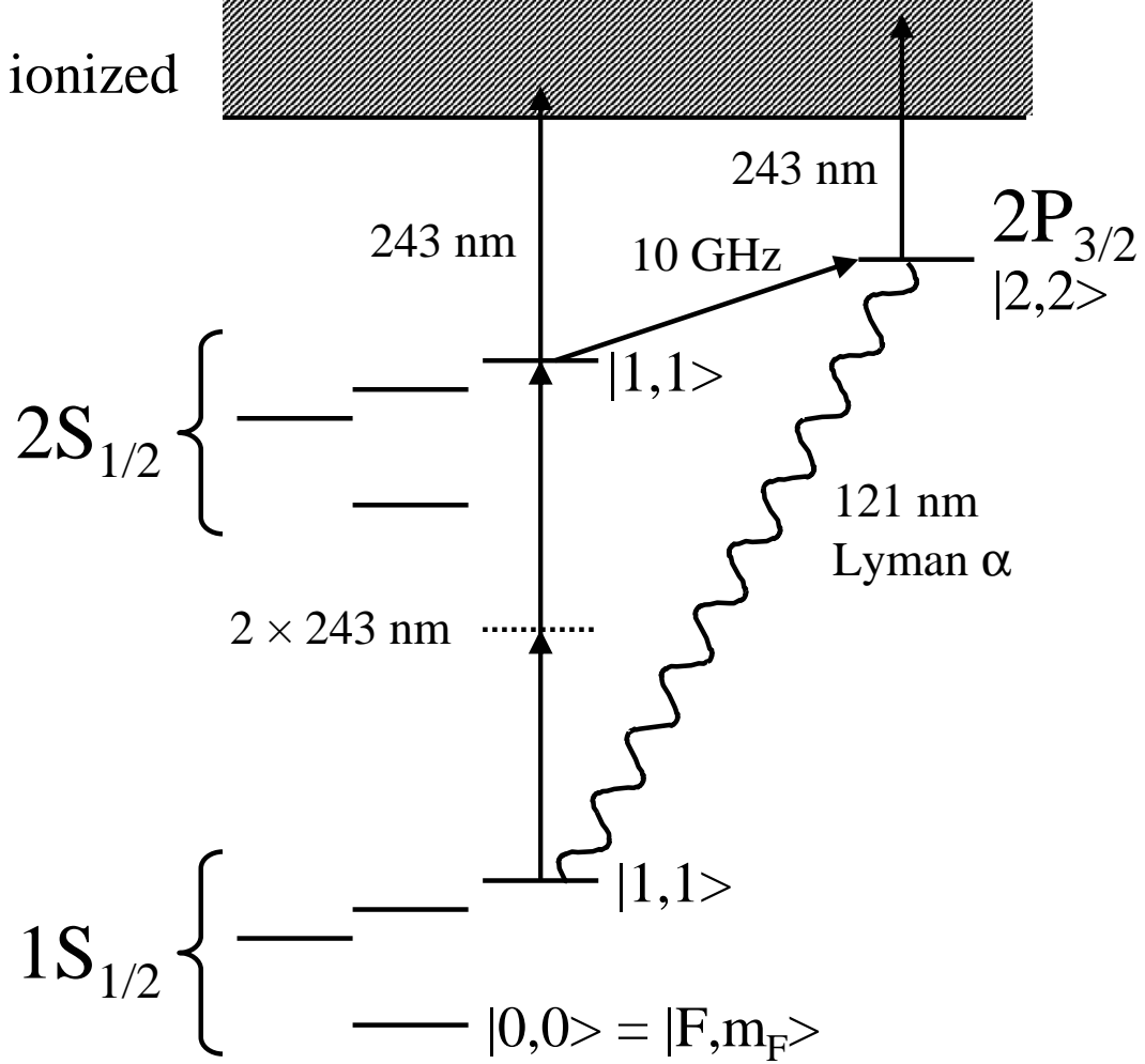
FIG. 3: Excitation scheme for laser cooling of magnetically trapped H or \bar{\text{H}} . The 243 nm light excites the atoms from the magnetically trapped 1S_{1/2} |F, m_F\rangle = |1, 1\rangle state to the 2S_{1/2} |1, 1\rangle state. Radiation near 10 GHz quenches the metastable 2S state to the 2P_{3/2} |2, 2\rangle state. The atoms reradiate on the 1S_{1/2} |1, 1\rangle - 2P_{3/2} |2, 2\rangle transition at 121 nm, returning to the magnetically trapped state. While in the 2S_{1/2} or 2P_{3/2} state, an atom can be photoionized by a single 243 nm photon. For clarity, only the relevant 2P_{3/2} substate is shown.
