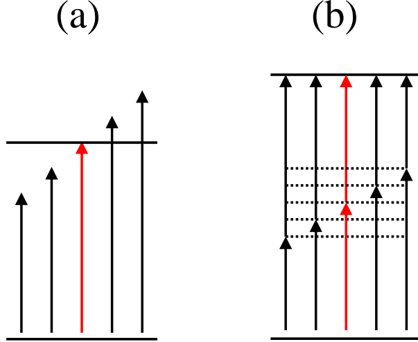
FIG. 2: Comparison of mode-locked and CW excitation of (a) single-photon and (b) two-photon transitions using energy-level diagrams. In (a), the frequency comb of the mode-locked laser (black) has only one component resonant with the atomic transition, while all the CW light (red) is resonant. In (b), we show a two-photon transition for which all intermediate states are far from single-photon resonance. The mode-locked laser induces many transition paths whose amplitudes add coherently, while the CW light follows only one path. The two-photon transition rates turn out to be roughly equal for equal average power.
