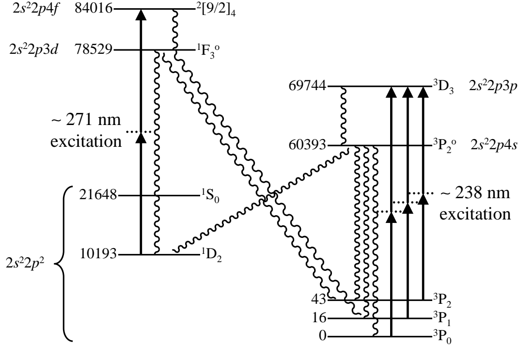
FIG. 4: Energy level diagram for laser cooling of carbon. Energies of states are given next to the horizontal line denoting the state, and are measured in \text{cm}^{-1} above the lowest-energy state. Laser excitation is shown by solid vertical lines, radiative decay by wavy lines. Shaded boxes denote portions of the radiative decay paths that are not involved in laser excitation, and are labeled as belonging to the singlet or triplet manifold.
