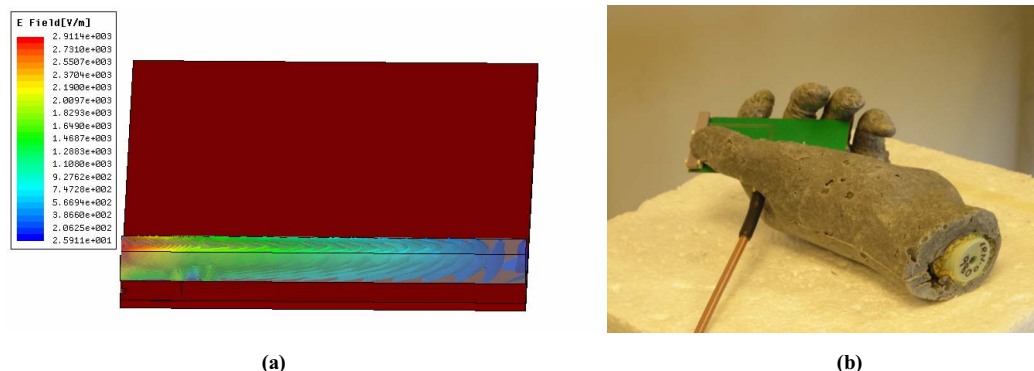
Fig. 2 (a) Simulated Electric Field inside the dielectric (b) PD-PIFA mounted in the phantom hand
