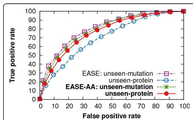
Figure 1 ROC curves performance of EASE and EASE-AA using two different evaluation schemes. The true positive rate of EASE and EASE-AA is shown as a function of the false positive rate at different prediction thresholds. These are independent test results using the unseen-mutation and unseen-protein evaluation. While for EASE-AA the area under the ROC curve (AUC) declined only by 0.02 when comparing the unseen-mutation and unseen-protein evaluation, EASE yielded a decrease of 0.11.
