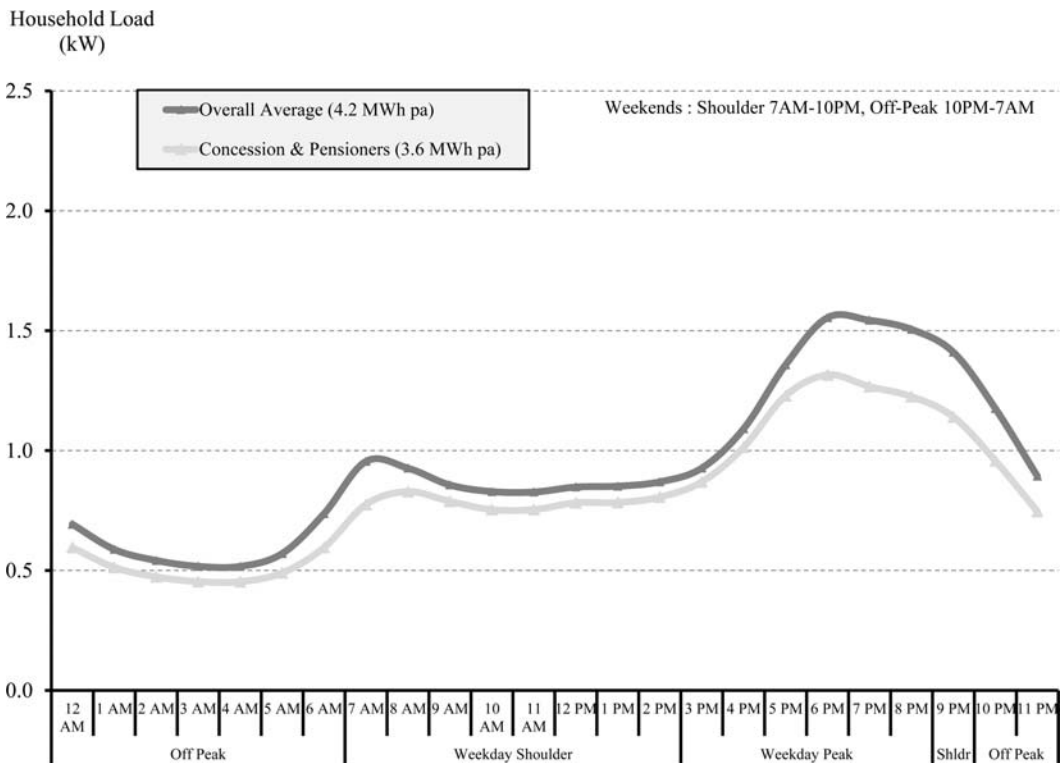
Figure 7: Annual Average Weekday Load Curve: Concession & Pensioner Households
