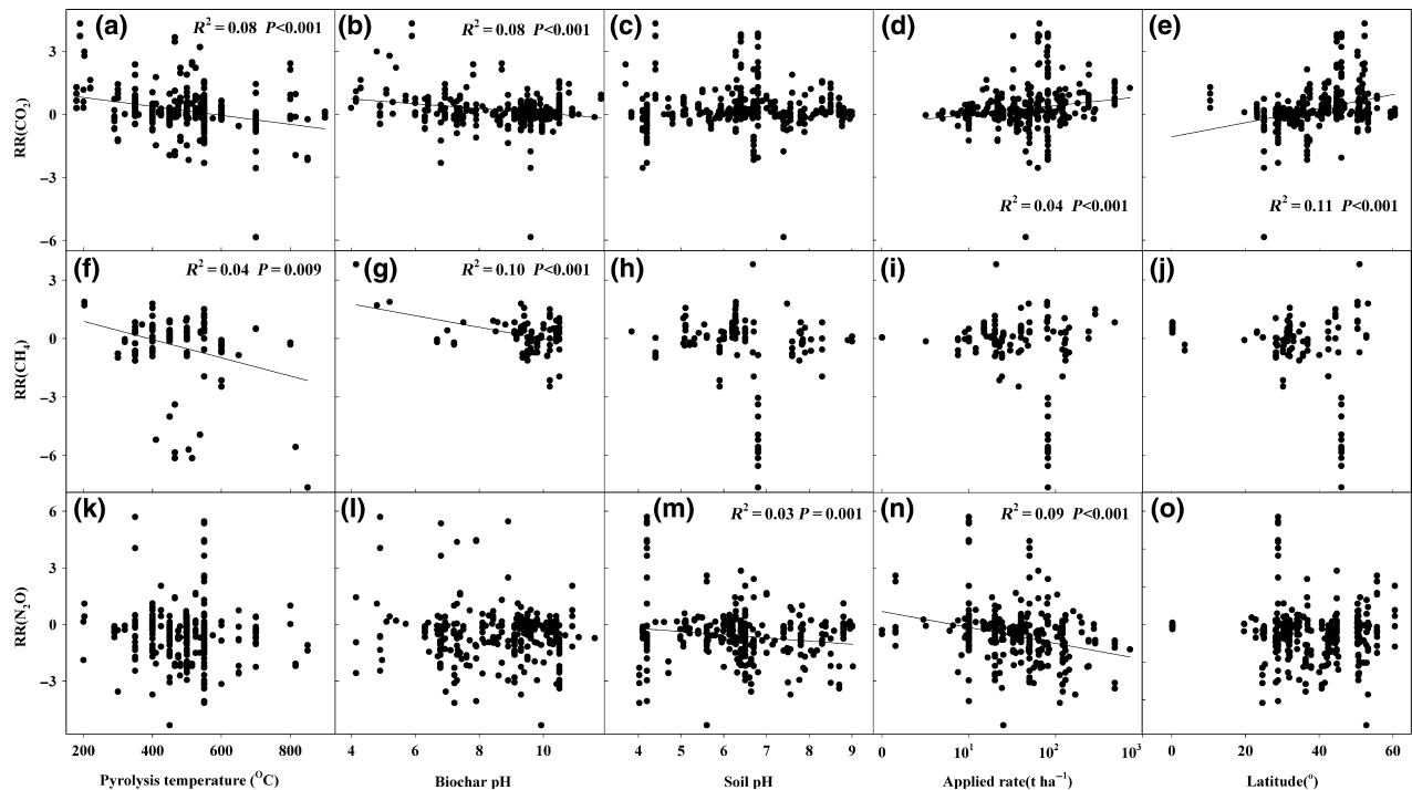
Fig. 4 Effects of biochar pyrolysis temperature, biochar pH, soil pH, applied rate, and latitude on response ratios of soil CO 2 emissions (a–e), CH 4 emissions (f–j), and N 2 O emissions (k–o) to biochar application.
