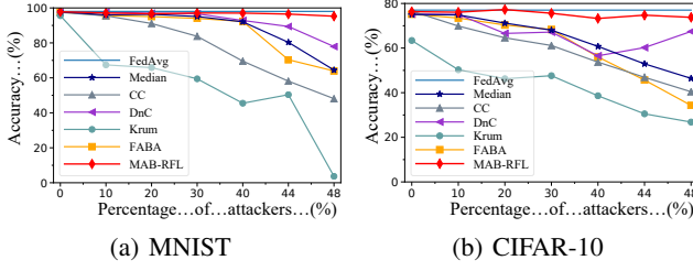
Figure 3: Model accuracy under label flipping attack
