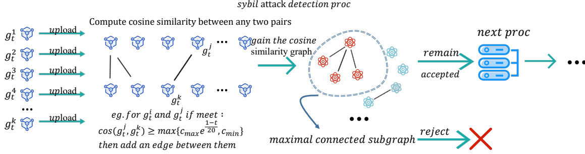
Figure 2: Illustration of sybil attack detection
