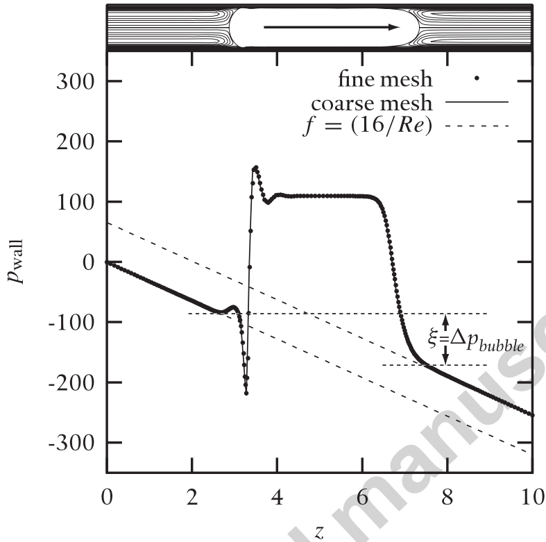
Figure 3: Wall pressure distribution of a unit cell in gas-liquid Taylor flow in the axial direction for Ca = 0.01 and Re = 100 . Dynamic holdup of the liquid (the fraction of channel length occupied by the liquid) in the channel is 0.65 and dimensionless length is 10 (Kreutzer et al. (2005b)).
