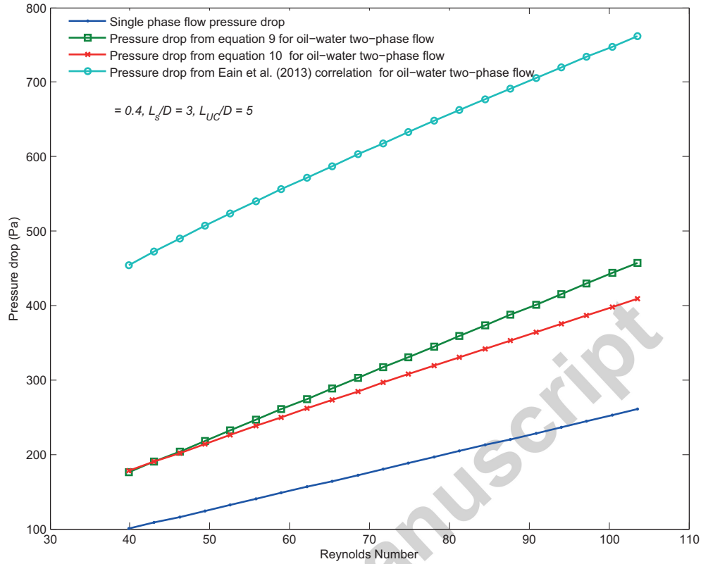
Figure 4: Variation of pressure drop with Reynolds number in a circular microchannels of diameter 800\mu\text{m} with a length of 50D based on different pressure drop correlations from the literature (equation 9, equation 10 and correlation in Eain et al. (2013)). The data points are generated using the values and relationships shown in the Table 3 for a liquid-liquid two-phase flow with water as primary fluid and silicon as secondary fluid.
