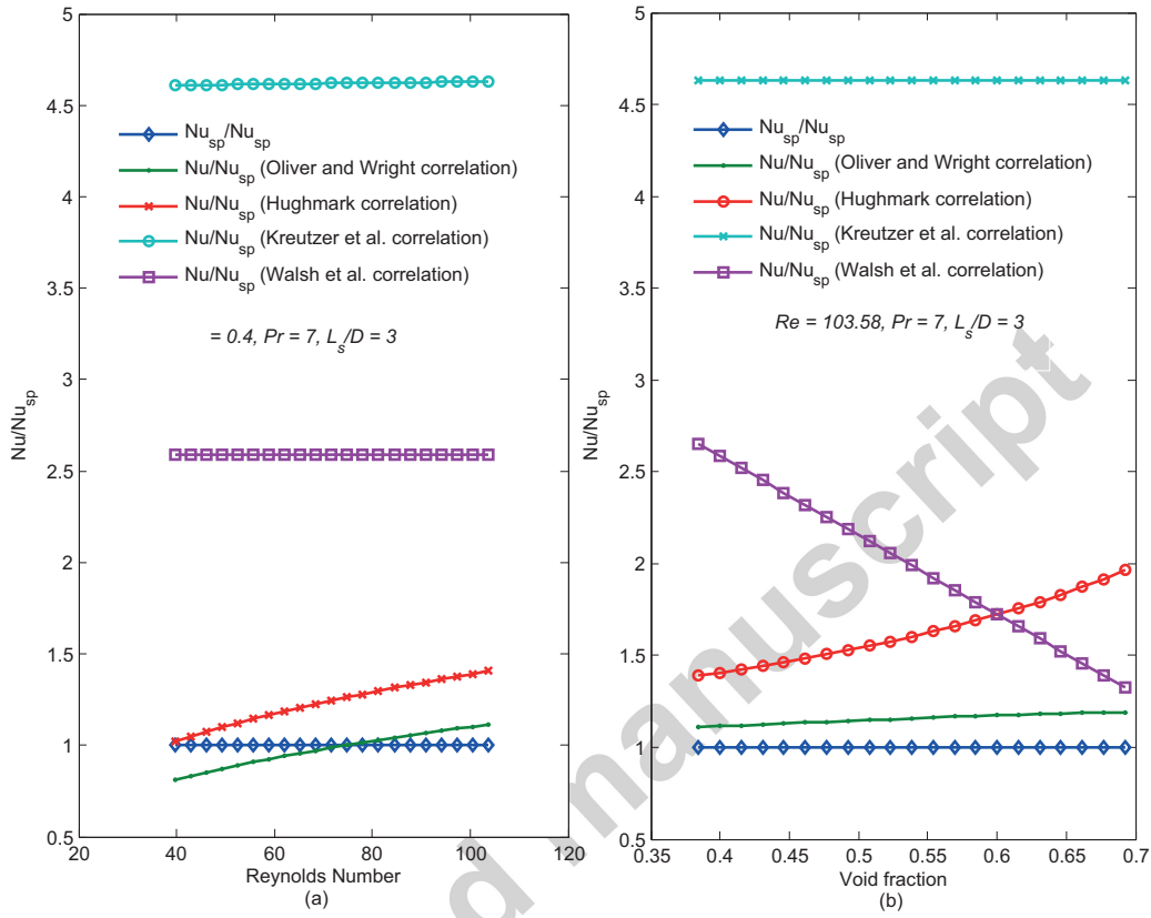
Figure 7: Variation of Nusselt number (nondimensionalized with respect to single phase) with Reynolds number and void fraction in a circular microchannels of diameter 800\mu\text{m} based on different correlations from the literature (Oliver and Wright (1964); Hughmark (1965); Kreutzer et al. (2001); Walsh et al. (2010)). The parameters (ratio of flow rates and slug lengths) are selected arbitrarily for a liquid-liquid two-phase flow with water as primary fluid and silicon oil as secondary fluid. The data points are generated using the values and relationships shown in the Table 3
