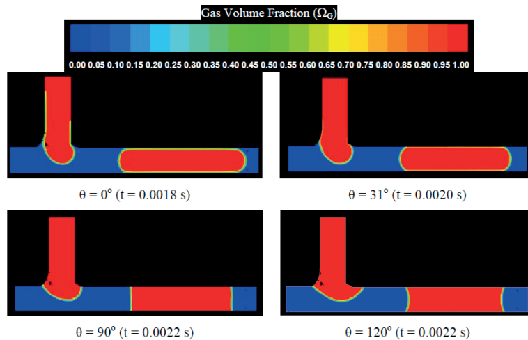
Figure 6: Effect of contact angle on slug formation in gas-liquid two-phase flow in a T-junction (Using CFD) (Santos and Kawaji (2010)).
