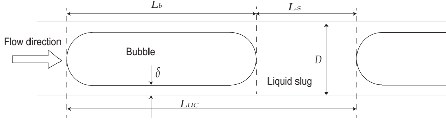
Figure 2: Schematic diagram of a two-phase flow unit cell of slug and bubble.
