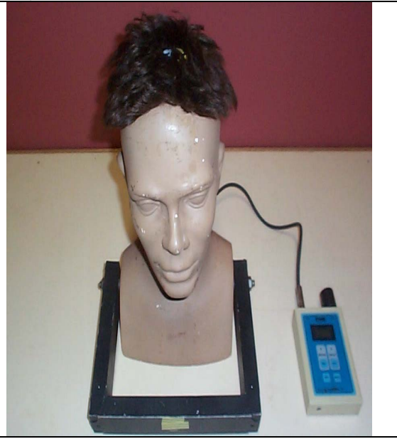
Figure 1 - The setup of the head form and sensor without a hair piece (A) and with a hair piece (B).
