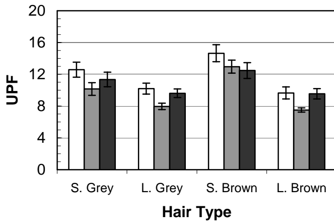
Figure 4 – The UPF averaged over the range of SZA for each hair type in full sun with the head upright, the head in shade with the head upright and the head in sun and pointed towards the sun. The error bars represent \pm one standard error.
