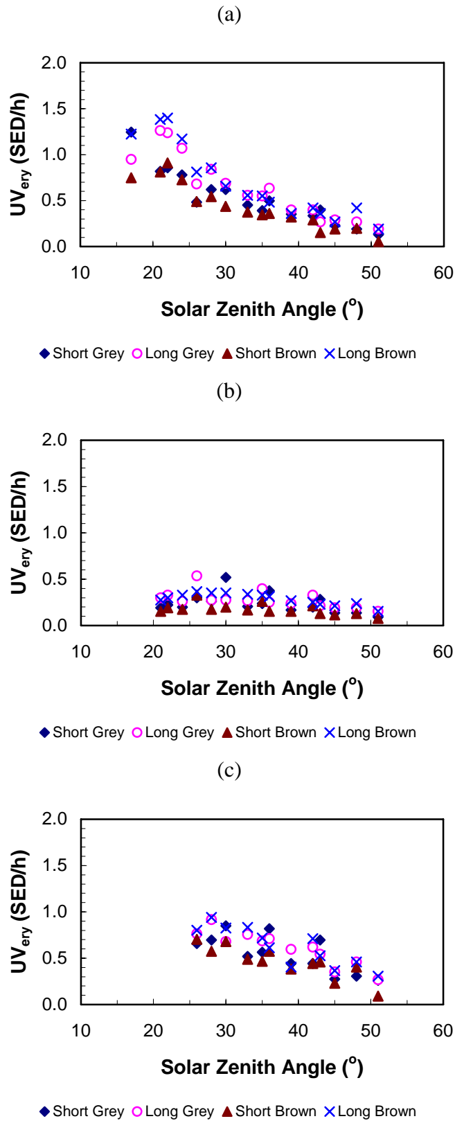
Figure 2 – The erythemal irradiances in units of SED/h to the scalp through the hair for (a) an upright head in full sun, (b) an upright head in shade and (c) a head in full sun and oriented in the direction of the sun.
