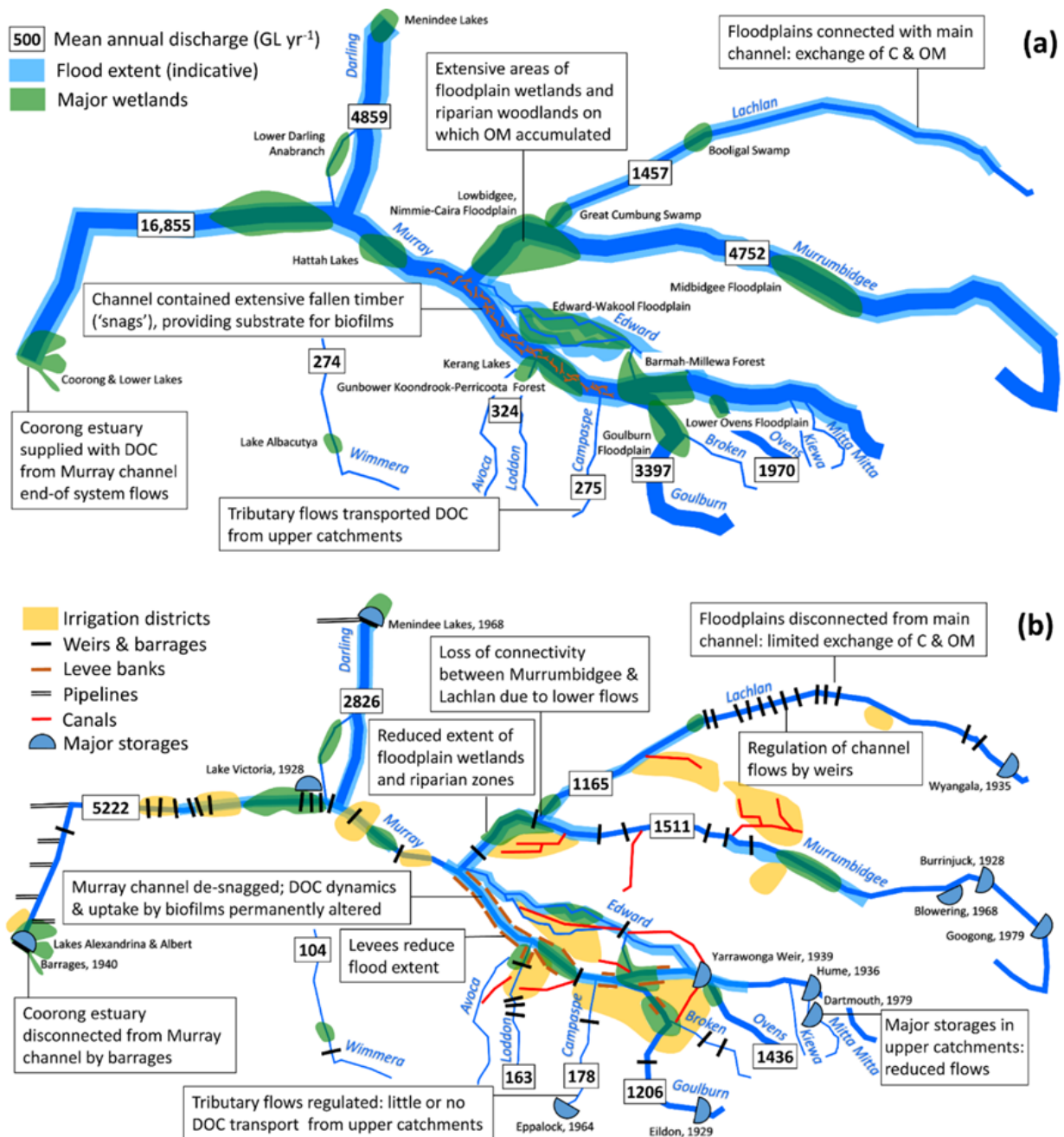
Figure 2. Changes in water available for the environment (inflows minus diversions) and carbon dynamics of rivers, floodplains and wetlands of the southern Murray-Darling Basin under (a) no water resource development and historical climate (1985-2006); (b) current water resource development, recent climate (1997-2006). Flow data from CSIRO (2008; Appendix A therein). OM = organic matter; DOC = dissolved organic carbon
