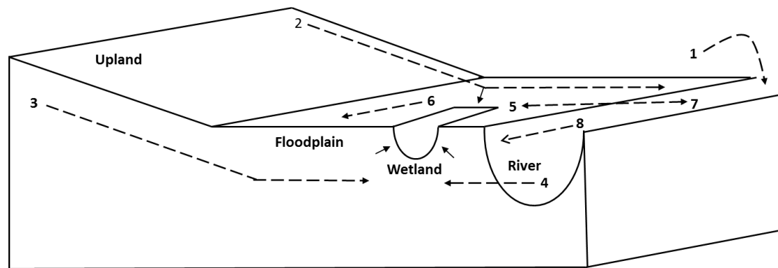
Figure 3. Schematic representation of flow paths in a lowland river–floodplain ecosystem. Litter fall (Pathway 1); overland flow from uplands during rain events (Pathway 2); sub-surface flows from the floodplain to the river (Pathway 3); sub-surface flows from the river channel to the floodplain (Pathway 4); lateral movement from the river to the floodplain during overbank flows (Pathway 5); longitudinal flows along the floodplain during flooding (Pathway 6); overbank return flows (Pathway 7); longitudinal flows in the river channel (Pathway 8)
