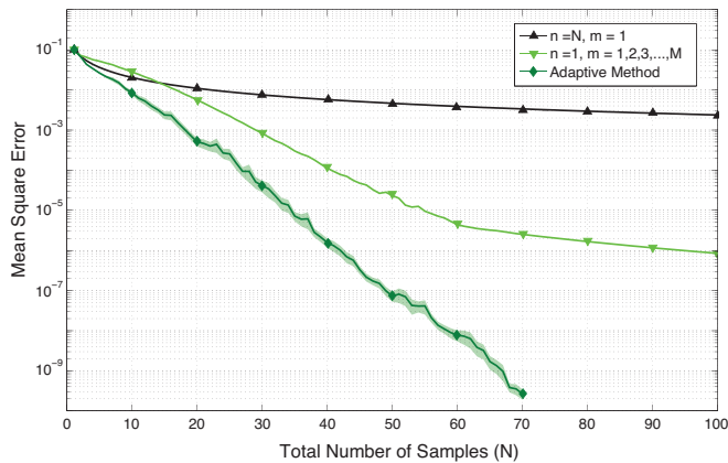
FIG. 3: The plots for mean square error as a function of the total number of measurements: ( \blacktriangle ) the Bayesian method where the N samples are taken at m = 1 ; ( \blacktriangledown ) the Bayesian method where the N samples are sequentially taken at times m = 1, 2, 3, \dots, M ; ( \blacklozenge ) the locally optimal adaptive strategy. The average MSE was computed from 10 000 simulations and the largest possible allowed waiting time was m_{max} = 1000 . The shaded region on the adaptive strategy plot represents the standard deviation of the MSE.
