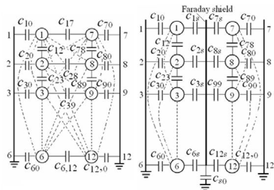
(a) Without Faraday shield, (b) With Faraday shield.
