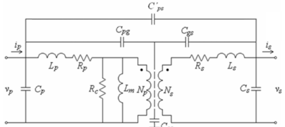
(b) with shield
