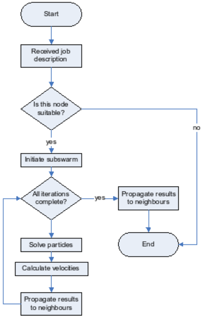
Fig. 1. Flowchart for main P2P particle swarm algorithm loop. This procedure is executed independently on all nodes which receive the job description from the initiating node.
