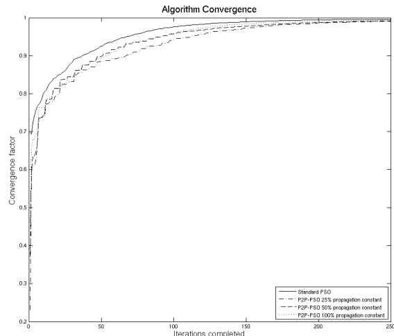
Fig. 2. Algorithm convergence for propagation constants of 25%, 50% and 100%, with traditional synchronous PSO performance provided for comparison.
