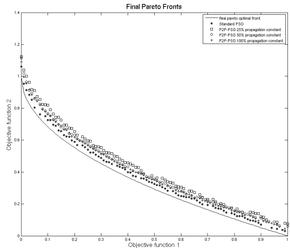
Fig. 3. Final Pareto-front approximations provided by the various PSO implementations.
