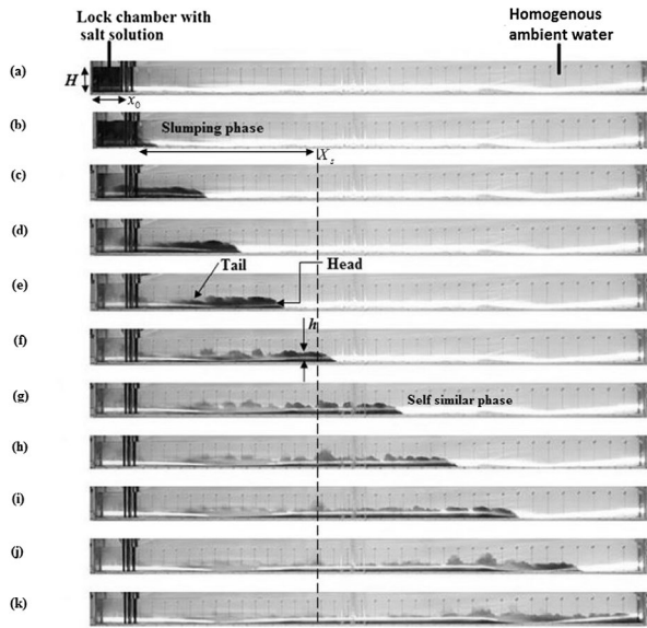
Figure 1. Phases of a lock-release gravity current (following the style of 8) (the non-uniform white streak is due to the LED backlighting and the crippled baking paper in front of the LED strip, this did not affect the data analysis).
