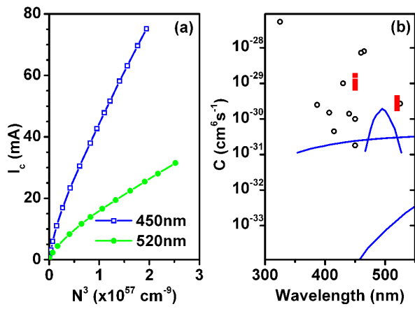
FIG. 4. (a) The Auger current I_c as defined in equation 6, plotted against N^3 for 44\mu\text{m} diameter 450nm emitting and 54\mu\text{m} diameter, 520nm emitting devices. The Auger coefficient C is given by the slope of this graph. (b) Values of the Auger coefficient C found in this work, and reported in the literature. The red squares show the values of C obtained from the work presented here; each symbol represents the value of C obtained from an individual device. Black open symbols denote experimental 6,7,25 determinations of C found in the literature, while the blue lines show reported theoretical 26 values for C .
