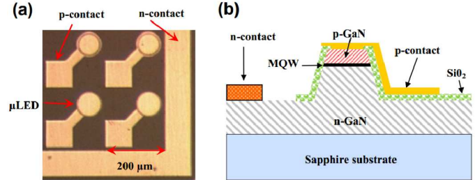
FIG. 1. (a): Plan view micrograph, showing four four representative \mu\text{LEDs} . (b): Schematic cross-section of the device structure used.
