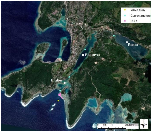
Figure 1 - In-situ instruments deployed within Erakor coral lagoon system.
