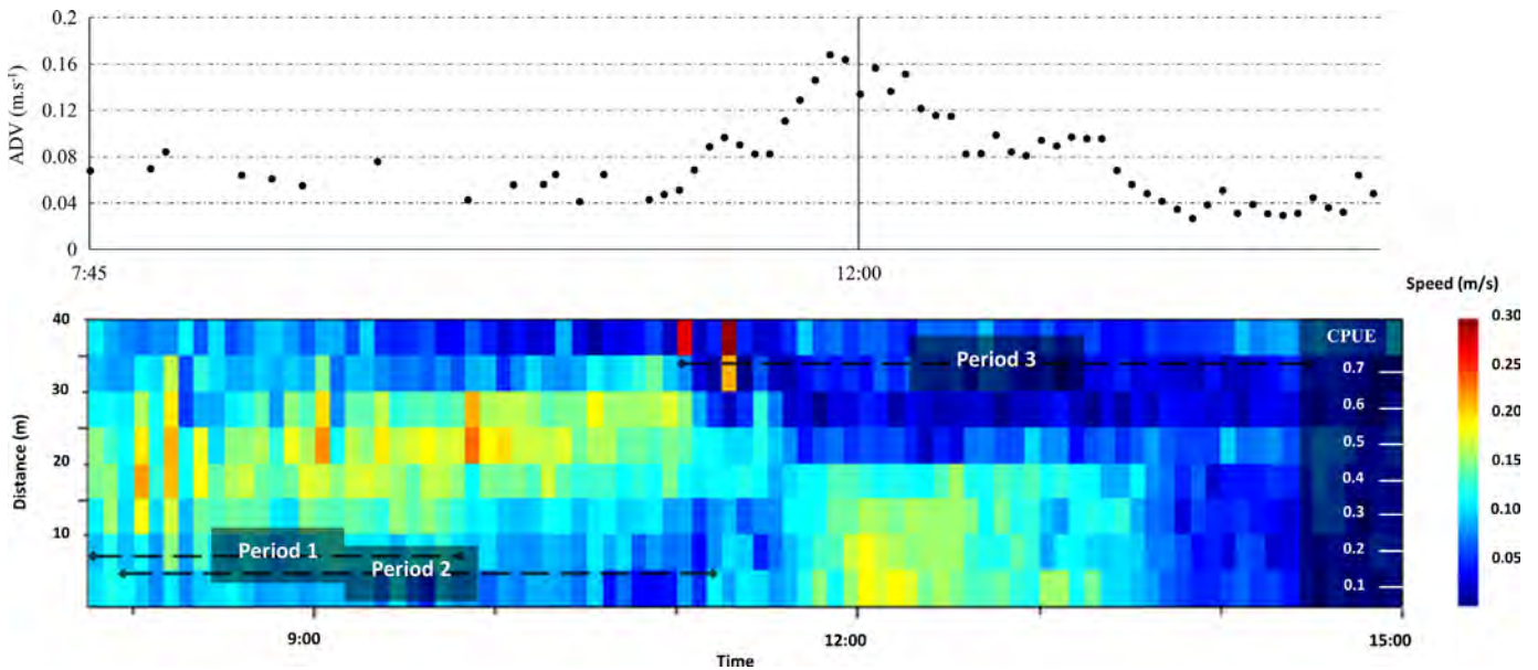
FIGURE 4. Time series of acoustic Doppler velocimeter (ADV; top) and acoustic Doppler current profiler (ADCP; bottom) data on day 3 (see Table 1). Gaps in the ADV time series are the result of removing erroneous data. The ADCP profile is shown as a function of current speed above the sensor head (~2.5 m above the seabed). The placement of “Period (1, 2, or 3)” denotes the mean CPUE (kg/net-hour; secondary y-axis) and soak time (length of the line relative to the x-axis) from each fishing period. Each row of rectangles represents the current speed (m/s) averaged over 5-m bins of the 40-m profile every 5 min.
