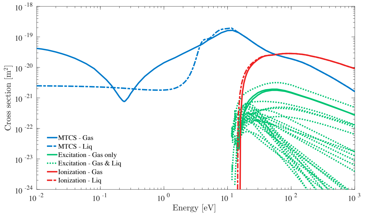
Figure 1. Gas and liquid argon electron scattering cross sections utilized in this study. Gas cross section data of Hayashi [55] via www.lxcat.net . Liquid cross section data of Boyle et al. [16] and necessary modifications of Hayashi set detailed in Section 2.2.1.
