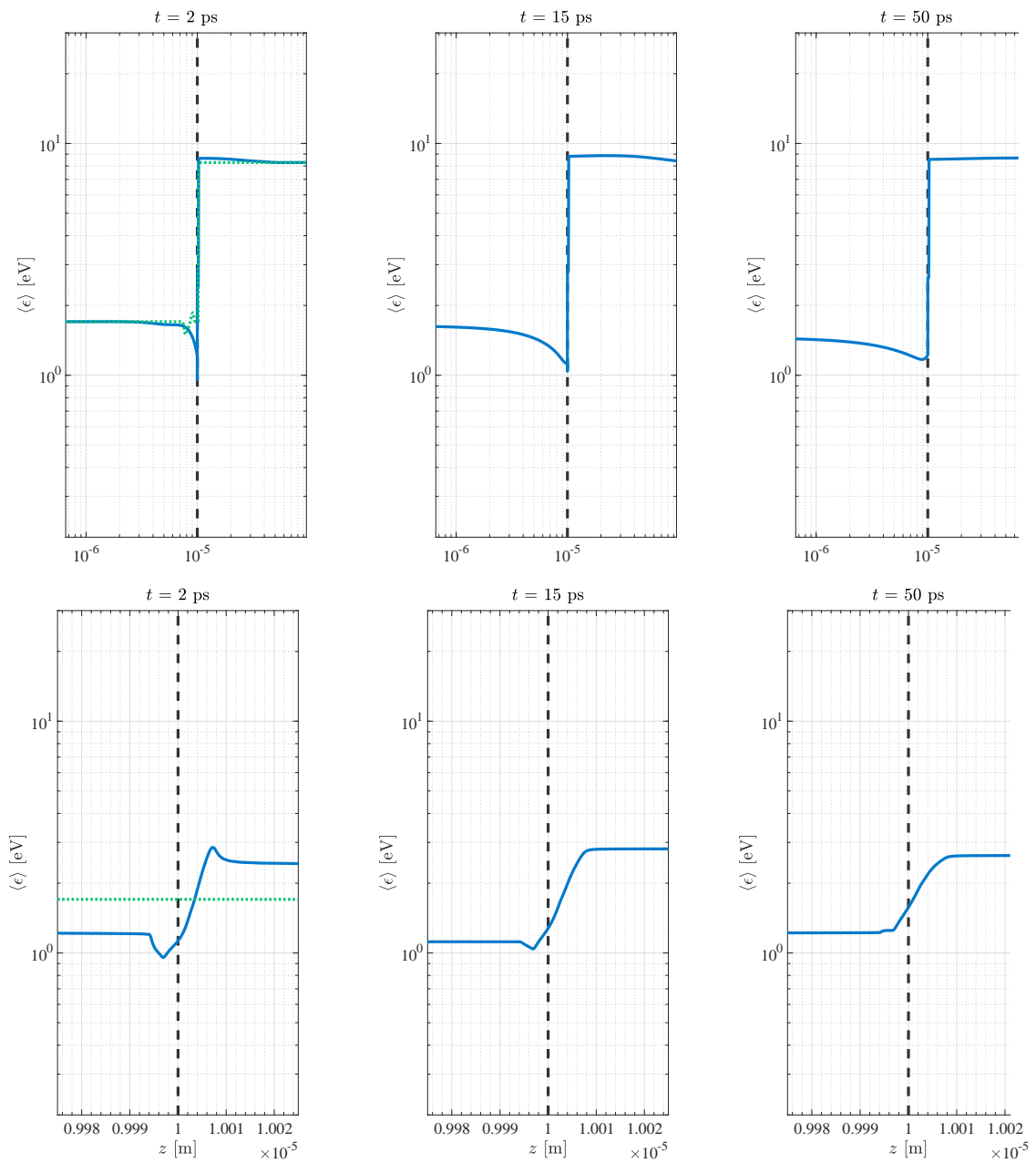
Figure 9. Electron mean energy for 4MM model at short, intermediate, and longer times as the electron swarm propagates from liquid to gaseous argon. Top view: Macroscopic results. Bottom view: Expanded view of interfacial results. Initial condition given by green dash-dot green line. Direction of field-driven propagation is from left to right.
