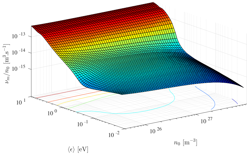
Figure A2. Reduced momentum transfer collision frequency, \frac{\nu_m}{n_0} , surface of electrons in argon computed via (A.11) as a function of \langle\epsilon\rangle and n_0 used to interpolate input data for the 4MM model.
