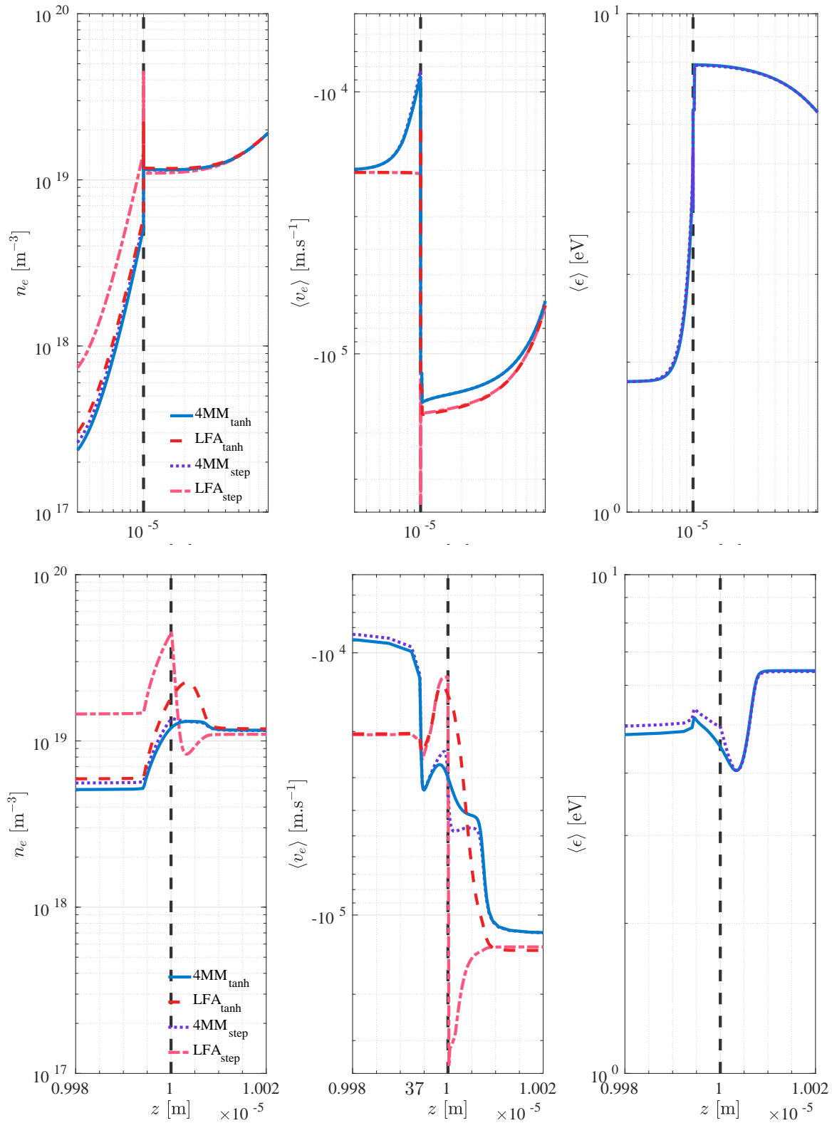
Figure 10. Electron density, average velocity and mean energy for 4MM and LFA models after 50 ps of an electron streamer penetrating from gaseous to liquid argon. Results of assuming a tanh or step function interface on are shown for comparison. Top view: Macroscopic results. Bottom view: Expanded view of interfacial results. Direction of field-driven propagation is from right to left.
