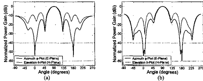
Fig. 2. Far-field radiation pattern of the original antenna (a) and reference antenna (b)
