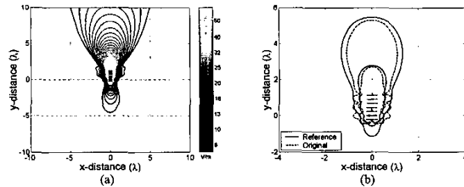
Fig. 3. (a) Near-field field-strength contour of the 7-element Yagi-Uda reference antenna calculated using Huygen's wavelets technique; and (b) Occupational (inner lines) and non-occupational (outer lines) E-field exposure zone boundaries calculated using Huygen's wavelets technique (solid lines) and NEC (dashed lines)
