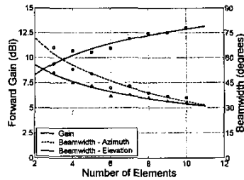
Fig. 1. Lookup curves for gain and half-power beamwidths
