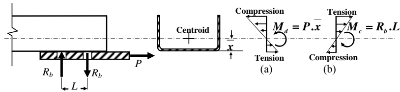
Figure 4 Effects of connection eccentricity \bar{x} and connection length L
