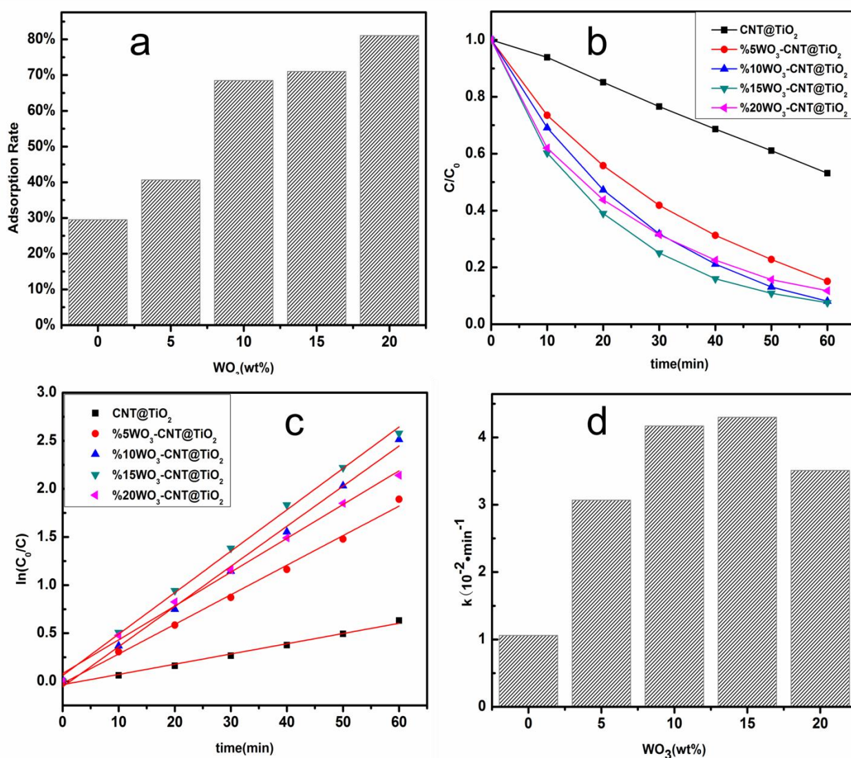
Fig 5 Photocatalytic degradation of MB using different samples as catalysts: (a) the adsorption abilities (b) photodegradation (c) reaction kinetic curves (d) the reaction rate constant (k) values comparison.
