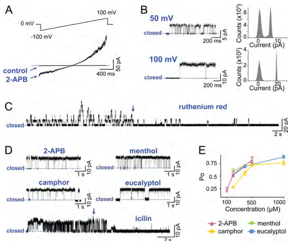
FIGURE 4. Functional reconstitution of purified hTRPV3. A , representative current recording from a planar lipid bilayer containing a high number of hTRPV3 channels during a ramp voltage protocol from -100 to 100 mV. Arrows , traces before (control) and after the addition of 100 \mu\text{M} 2-APB. Dashed line , zero current level. B , representative current traces of single-channel activity recorded from a planar lipid bilayer clamped at 50 and 100 mV after the addition of 100 \mu\text{M} 2-APB ( left ). The closed channel current level is indicated by dashed lines . Shown are corresponding current amplitude histograms ( right ), yielding a single-channel conductance of 174 pS. C , representative current trace from a lipid bilayer containing multiple hTRPV3 channels recorded at 100 mV. The channels were activated by 100 \mu\text{M} 2-APB and subsequently inhibited by 10 \mu\text{M} ruthenium red. The arrow indicates where ruthenium red was added. D , representative current traces of single-channel activity recorded at 100 mV in the presence of 100 \mu\text{M} 2-APB, 200 \mu\text{M} menthol, 500 \mu\text{M} camphor, or 500 \mu\text{M} eucalyptol. The bottom trace shows inhibition of 2-APB-activated current by 10 \mu\text{M} icilin. The arrow indicates where icilin was added. E , scatter plot showing open probability ( P_o ) versus applied concentration of the tested agonists. Error bars , S.E.
