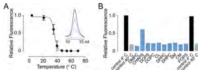
FIGURE 3. Thermostability-based FSEC screening for hTRPV3-stabilizing additives. A , melting curve of hTRPV3-GFP, yielding a melting temperature (i.e. the temperature at half-maximal fluorescence amplitude) of 36.2 \pm 1.0 °C. Relative fluorescence is calculated from oligomeric peak amplitudes in consecutive FSEC runs with hTRPV3-GFP samples, preheated at different temperatures. Data represent mean \pm S.E. (error bars) ( n = 3 ). Inset , overlay of the oligomeric peak FSEC profiles. B , bar diagram shows relative fluorescence of oligomeric peak amplitudes from consecutive FSEC runs with a selection of additives tested for possible stabilizing effects on hTRPV3-GFP. Black and gray bars represent relative FSEC peak amplitudes of hTRPV3-GFP without additives, incubated at 4 and 40 °C, respectively (with control 4 °C set as 1). Blue bars , relative peak amplitudes of hTRPV3-GFP samples supplemented with various additives before incubation at 40 °C.
