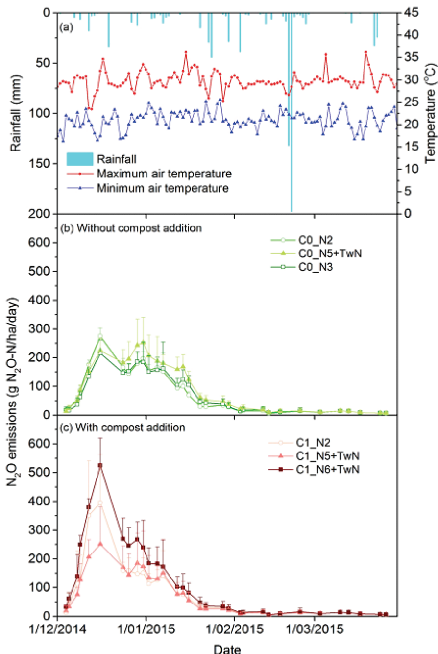
Fig. 3—(a) Daily rainfall and air temperature in relation to N_2O emission dynamics; (b) for treatments without compost addition and (c) with compost addition in the third ratoon.
