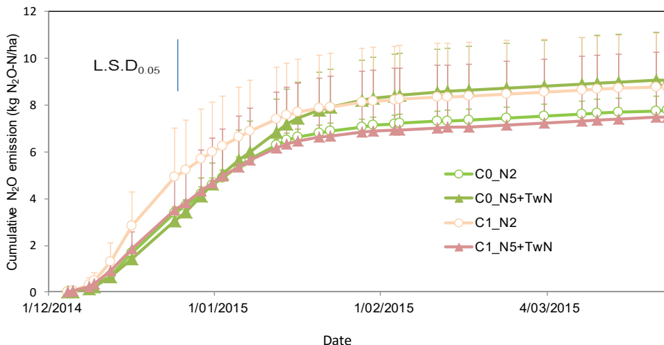
Fig. 4—Effects of compost and Twin N application on cumulative N 2 O emissions for the 147 kgN/ha rate (N2 and N5) in the third ratoon.
